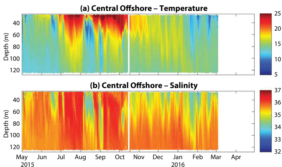
FIGURE 6. Temperature (°C) and salinity record from the central offshore wire-following profiler. Data are processed to hourly averages with vertical resolution of one meter.
