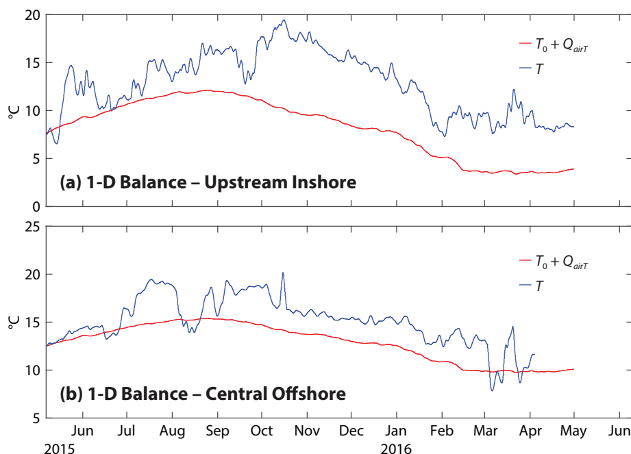
FIGURE 8. Depth-averaged temperature (blue) and the combination of initial temperature and cumulative air-sea heat flux (red) at inshore and central sites from May 2015 to April 2016. All units are °C.
