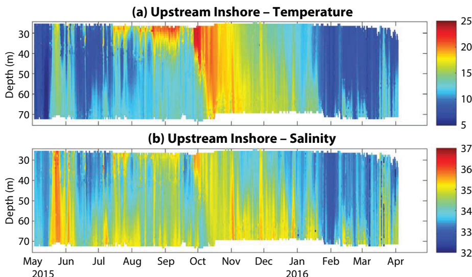
FIGURE 4. Temperature ( ^{\circ}\text{C} ) and salinity record from the upstream inshore wire-following profiler. Data are processed to hourly averages with vertical resolution of one meter.
