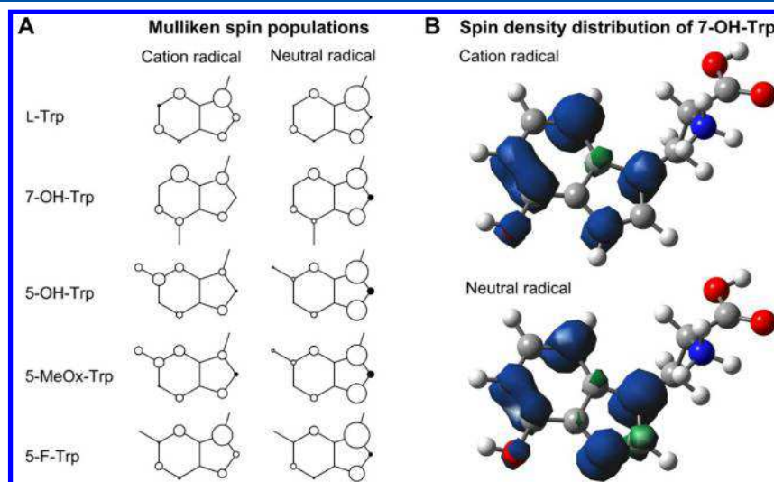
Figure 4. (A) Mulliken spin populations ( p -orbital \pi -component) for the radical forms of tryptophan derivatives. The open and solid circles symbolize positive and negative spin densities, respectively. The size of the circles represents the magnitude of the density. (B) Three-dimensional representation of the spin density distribution of cationic and neutral 7-OH-Trp radicals.
