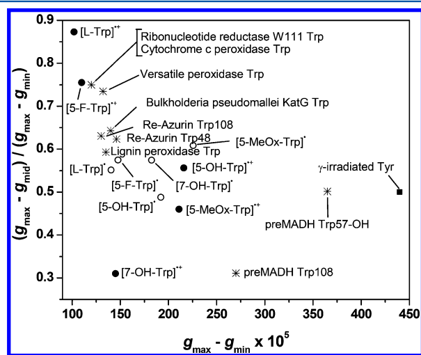
Figure 3. Plot of g -value anisotropy versus rhombicity of various tryptophan radical species. Tryptophan-based radicals measured in protein are represented by stars, cation radicals measured in this work are closed circles, and neutral radicals (as calculated in this study) are open circles. The y -axis shows rhombicity, where 1.0 and 0.0 would both be completely axial, and the x -axis shows g -value anisotropy, with 0 representing a purely isotropic signal.
