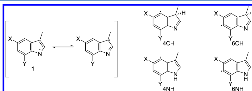
Figure 2. Potential neutral radical structures resulting from \pi -radical delocalization over the indole ring.
