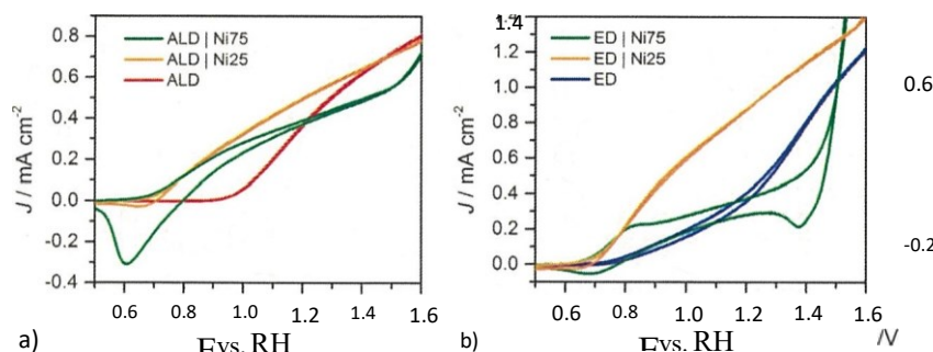
Figure 2. J–E curves measured at 20 mV under 1 sun illumination for bare and modified (a) ALD and (b) ED hematite electrodes in contact with 1 M KOH solution; bare ALD (red), bare ED (blue), Ni75 coated hematite (green), Ni25 coated hematite (orange). The dark current are not included for the sake of clarity and are shown in Figure S5.
