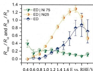
Figure 5. R trap /R ct for bare and R cat /R ct for catalyst modified ED electrodes; bare electrode (blue diamond), Ni 7 S modified ED electrode (green triangle), and Ni 2 S coated ED electrode (orange pentagon).
