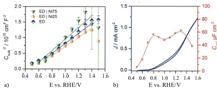
Figure 3. (a) MS plots for bare and catalyst modified ED electrodes, (b) J — E curve and C_{\text{cat}} values for bare ED electrode under 1 sun illumination in contact with 1 M KOH; bare electrode (blue diamond), Ni7S modified ED electrode (green triangle), and Ni2S coated ED electrode (orange pentagon). The dotted lines are the linear fitting used to extract the dopant density.
