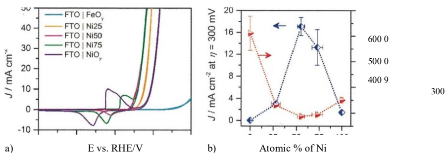
Figure 1. (a) IR-corrected CVs of \text{Ni}_x\text{Fe}_{1-x}\text{O}_y catalysts on FTO substrates; FeO (cyan), \text{Ni}_{0.25}\text{Fe}_{0.75}\text{O} (orange), \text{Ni}_{0.5}\text{Fe}_{0.5}\text{O} (pink), \text{Ni}_{0.75}\text{Fe}_{0.25}\text{O} (green), and NiO (purple). (b) Plots of current density at 300 mV overpotential (blue diamonds) and overpotential at 10 mA cm -2 (red triangle) as a function of the % Ni in contact with 1 M KOH; the compositions, activities, and the error bars are the average and standard deviations acquired from three independently prepared samples.
