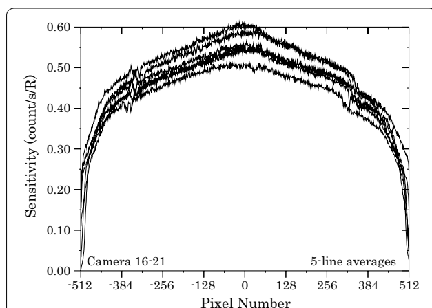
Fig. 4 Horizontal cross section of the sensitivities of the all-sky airglow/aurora imager #16–21 measured by an integrating sphere of NIPR
