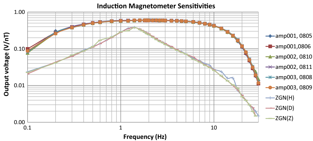
Fig. 7 Frequency dependence of sensitivities of the induction magnetometers
