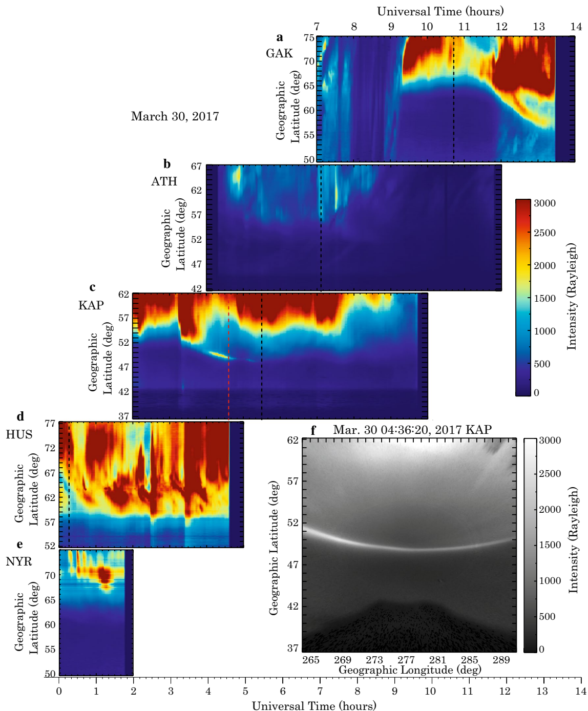
Fig. 5 North-south keograms of 630.0 nm emission (a–e) and an image (f) of 630.0-nm auroras obtained by the all-sky airglow/aurora imagers on March 30, 2017 at GAK, ATH, KAP, HUS, and NYR. They are shown in geographical coordinates. Black vertical dashed lines indicate the time of zero MLT. Red vertical dashed line in (c) is the timing when the image in (f) was taken
