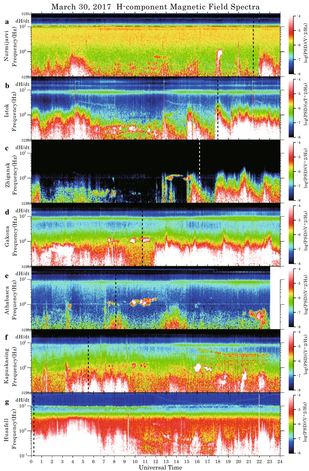
Fig. 9 One-day dynamic spectra of H-component magnetic field variations observed at seven stations around the north geomagnetic pole on March 30, 2017. Vertical dashed lines indicate 00 MLT (magnetic local midnight) at each station
