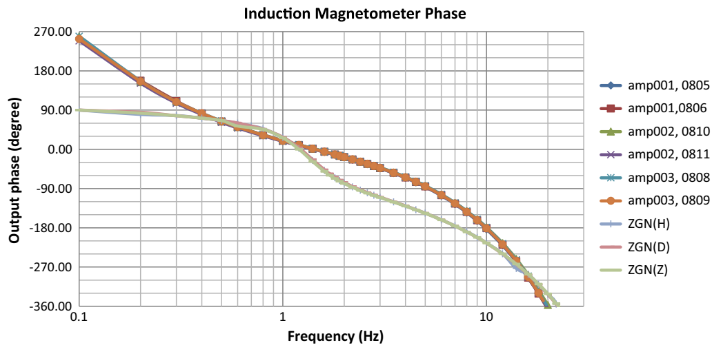
Fig. 8 Frequency dependence of phase of the induction magnetometers
