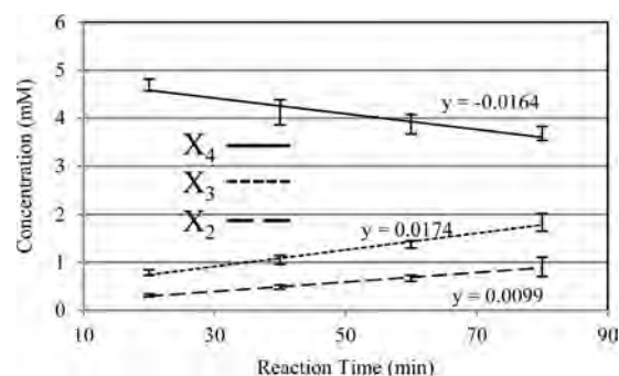
Figure 5. Hydrolysis of X 4 indicates substrate binding preference.
