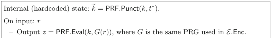
Fig. 14. Program C_{\tilde{k}} . This program replaces C_k . It is obfuscated and placed in the public key to be used for encryption.
