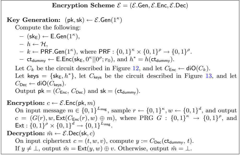
Fig. 11. One-time, bounded leakage encryption scheme, \mathcal{E} .
