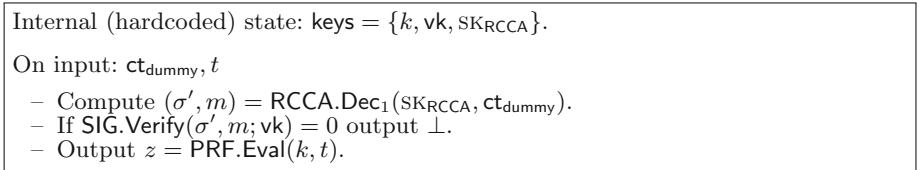
Fig. 19. Program C_{\text{keys}} . This program is obfuscated and placed in the public key. It is used during decryption.
