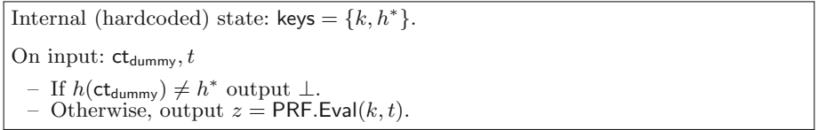
Fig. 13. This program C_{\text{keys}} is obfuscated and placed in the public key. It is used during decryption.
