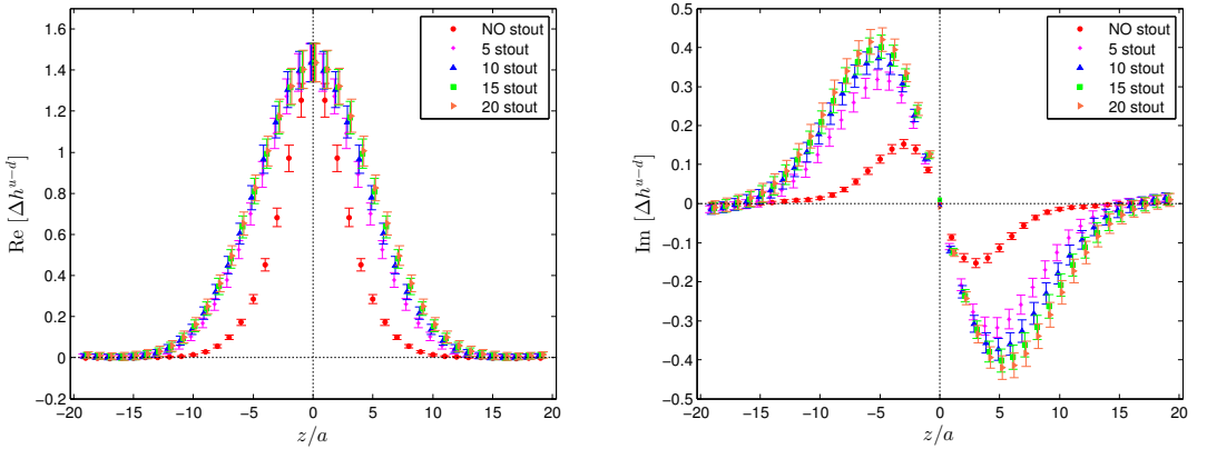
Figure 2. Real (left panel) and imaginary part (right panel) of the axial-vector form factors for different stout steps and |\vec{p}| = 6\pi/L .
