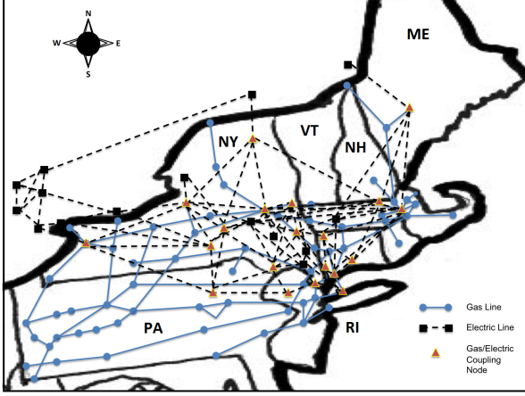
Figure 1: Network structure schematic of the CECE model for the US New England are: The IEEE 36-bus grid system and the Pennsylvania-to-Northeast gas system.
