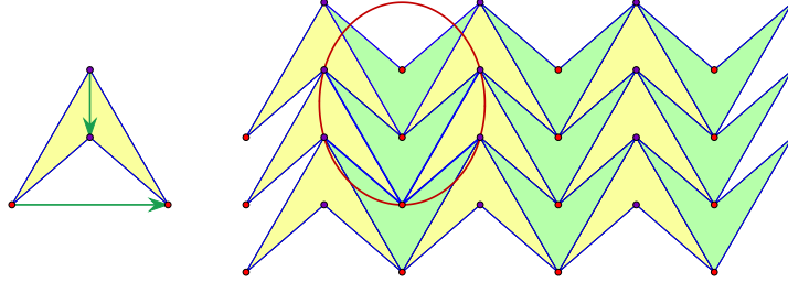
Figure 6: The double arrowhead framework can be generated from a single quadrilateral by adopting the diagonals as periods. The auxetic character is confirmed by the ellipse through one vertex and the endpoints of the four edges emanating from it.
