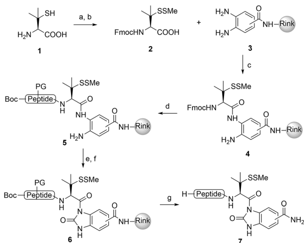
Scheme 1 Synthesis of peptidyl-Nbz. Reagents and conditions: (a) MMTS, EtOH, rt, 4 h; (b) Fmoc-Cl, TEA, CH 2 Cl 2 , rt, overnight; (c) 3 , DIC, oxyma pure, DMF, 8 h; (d) Fmoc-SPPS; (e) p -nitrophenylchloroformate, DCM, 40 min to 1 h; (f) DIEA, DMF, 15 min; (g) TFA/TIS/H 2 O (95 : 2.5 : 2.5). DMF = N,N -dimethylformamide, DIEA = N,N -diisopropylethylamine, HATU = 1-[bis (dimethylamino)-methyl-ene]-1 H -1,2,3-triazolo[4,5- b ]pyridinium 3-oxid hexa-fluorophosphate, DBU = 1,8-diazabicyclo[5.4.0]undec-7-ene, DIC = N,N -diisopropylcarbodiimide, oxyma pure = ethyl cyanoglyoxylate-2-oxime, TFA = trifluoroacetic acid, TIS = triisopropylsilane, and PG = protecting groups.
