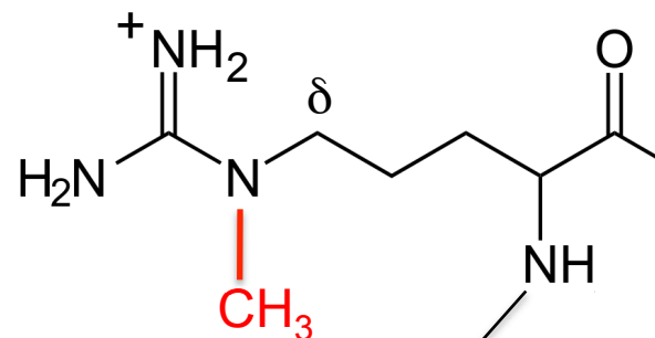
\delta - N -monomethylarginine
