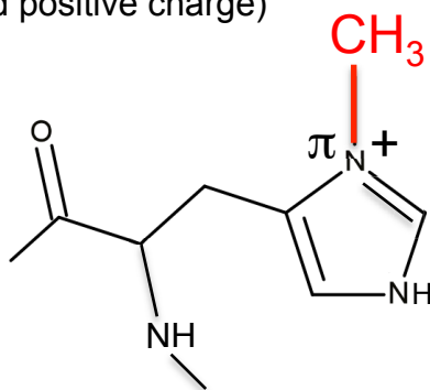
\pi - N -methylhistidine (1-methylhistidine in biochemical nomenclature but 3-methylhistidine in organic nomenclature)
