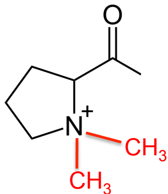
\alpha - N -dimethylproline (fixed positive charge)
