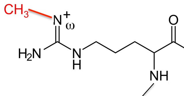
\omega - N -monomethylarginine
