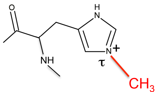
\tau - N -methylhistidine (3-methylhistidine in biochemical nomenclature but 1-methylhistidine in organic nomenclature)
