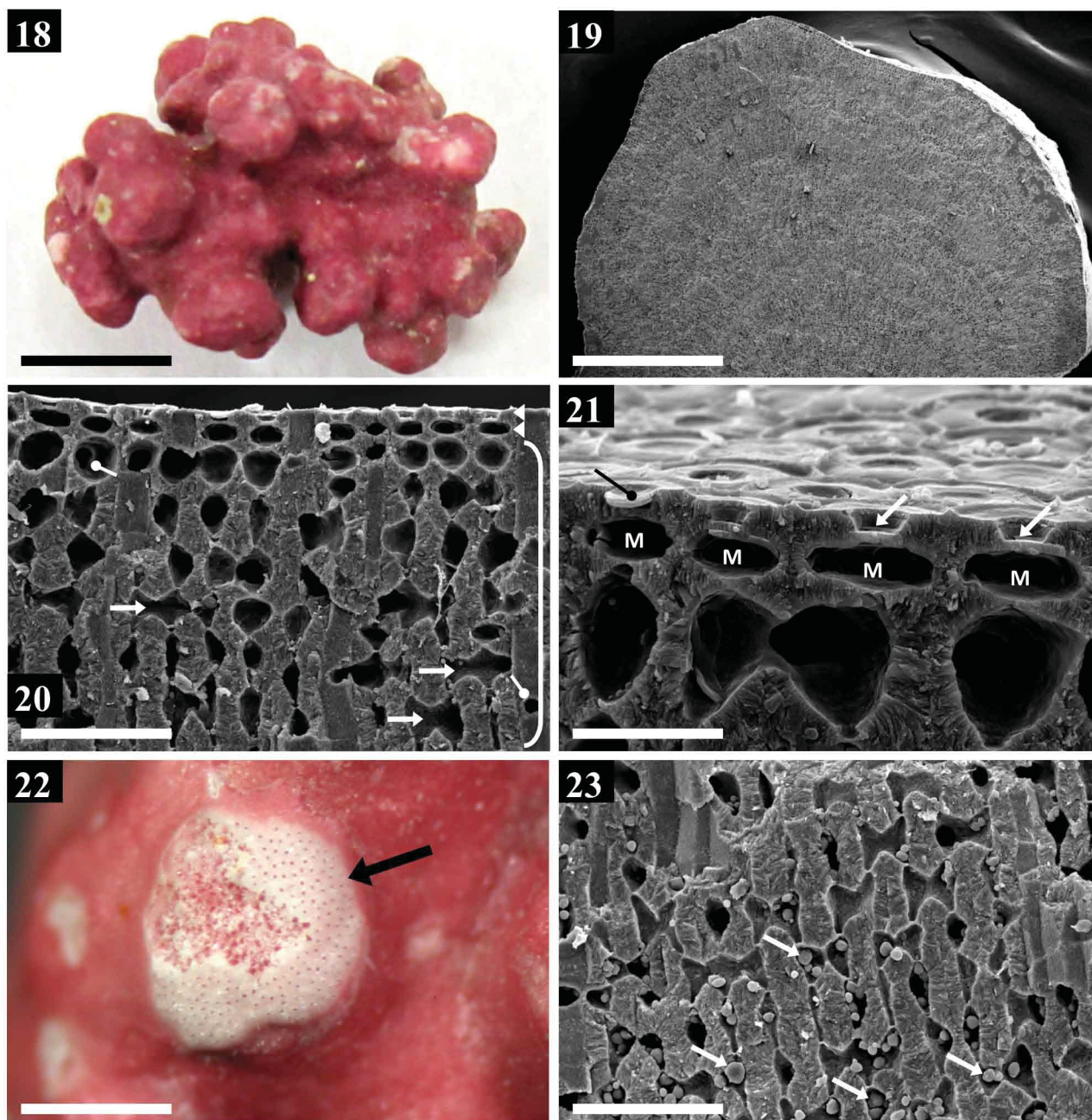
FIGURES 18–23. Specimen LAF 6970B. FIG. 18. Thallus habit showing numerous protuberances. Scale bar 6 mm. FIG. 19. Longitudinal section through protuberance showing perithallium with no overgrown tetrasporangial compartments. Scale bar 1.05 mm. FIG. 20. Epithallium (upper arrowhead), intercalary meristem (lower arrowhead) and perithallium (right bracket) showing cell fusions in the x-axis (arrows) and z-axis (circle pointers). Scale bar 4 \mu m. FIG. 21. Armored epithallial cells (arrows), one showing intact cell roof (circle pointer), and meristematic cells (M). Scale bar 14 \mu m. FIG. 22. Dissecting microscope view of thallus surface showing tetrasporangial sorus (arrow). Scale bar 1 mm. FIG. 23. Perithallium showing unidentified spherical inclusions (arrows), which may be unidentified life history stages of microalgal organisms. Scale bar 43 \mu m.
