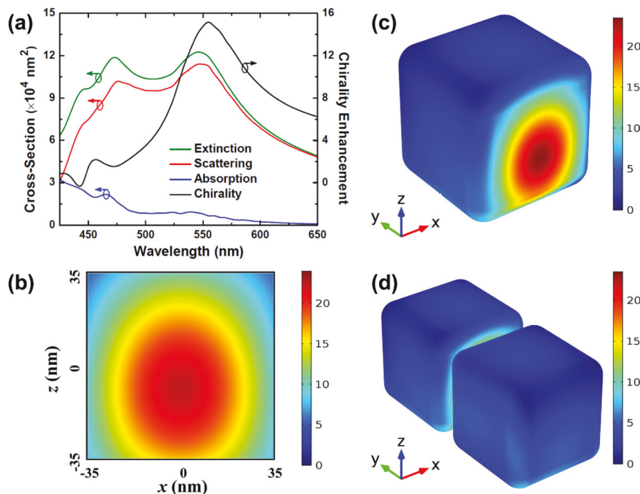
Fig. 2 Enhanced optical chirality in a silicon nanocube dimer. (a) Spectrum of volume-averaged chirality in the dimer gap (black) and spectra of the scattering (red), absorption (blue), and extinction (green) cross sections of the dimer under top illumination of an RCP plane wave. (b) 2D map of optical chirality density on the cutting plane through the gap center at 555 nm wavelength. (c, d) Surface distribution of optical chirality observed from the gap (c) and from the end (d). Only one nanocube in the dimer is shown in (c) for clarity.
