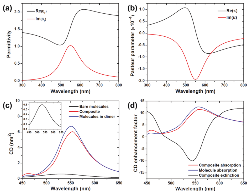
Fig. 5 Dispersion of permittivity \epsilon_c (a) and the Pasteur parameter \kappa (b) of the chiral molecules with typical extinction and CD values. (c) The CD absorption spectra for a chiral molecule slab with (red and blue curves) and without (black curve) the nanocube dimer. For the former, the CD signal is calculated in the whole composite (red) and in the chiral medium only (blue). Inset: zoom-in image of the CD for bare molecules. (d) The CD enhancement factor.
