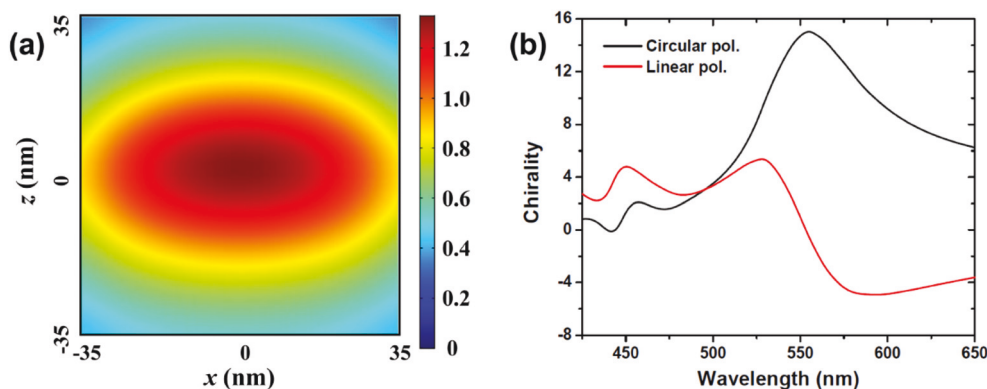
Fig. 6 (a) Distribution of the dissymmetry factor on the cutting plane through the gap center. (b) Comparison of volume-averaged chirality density in the dimer gap under the illumination of circularly (black) and linearly (red) polarized light.
