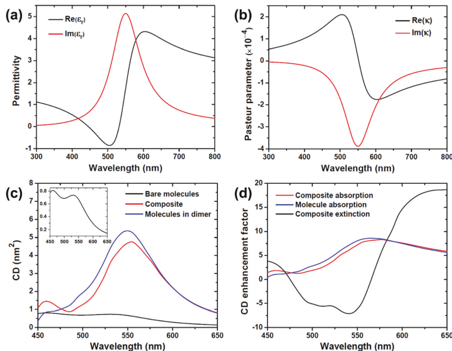
Fig. 4 Dispersion of permittivity \epsilon_c (a) and the Pasteur parameter \kappa (b) of the chiral molecules similar to bR. (c) The CD absorption spectra for a chiral molecule slab with (red and blue curves) and without (black curve) the nanocube dimer. For the former, the CD signal is calculated in the whole composite (red) and in the chiral medium only (blue). Inset: zoom-in image of the CD for bare molecules. (d) The CD enhancement factor.
