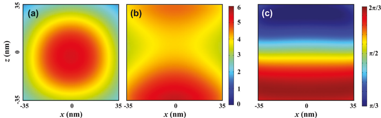
Fig. 3 2D maps of the magnetic (a) and electric (b) fields and their relative phase distribution (c) on the cutting plane through the dimer gap center. The field intensities show complementary patterns, which together with the relative phase close to \pi/2 satisfy all the conditions to maximize local optical chirality density.
