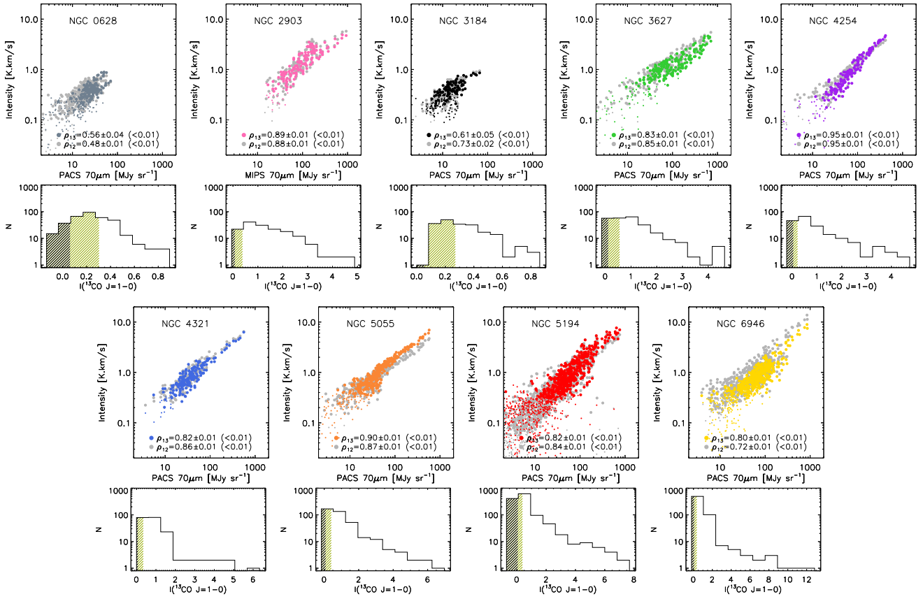
Figure 1. Top panels: EMPIRE observations of the CO line intensity (in K km s -1 ) on the y-axis following well the broadband 70μm intensity (in MJy sr -1 ) which is a proxy for the star-formation rate surface density on the x-axis. ^{13}\text{CO}(1-0) data are in colour and ^{12}\text{CO}(1-0) data, scaled by a factor of 10, are in grey. For both CO lines, smaller circles correspond to pixels below a signal-to-noise ratio of 5 in the respective maps. The Spearman's rank correlation coefficients between each CO line intensity and the 70μm intensity, their uncertainty, and their significance (in parenthesis), are indicated. Those are measured on data with signal-to-noise ratio above 5. Bottom panels: Histogram of the ^{13}\text{CO}(1-0) intensities. Only few pixels are below the 1σ (5σ) noise level as indicated by the hashed black (beige) parts of the histograms.
