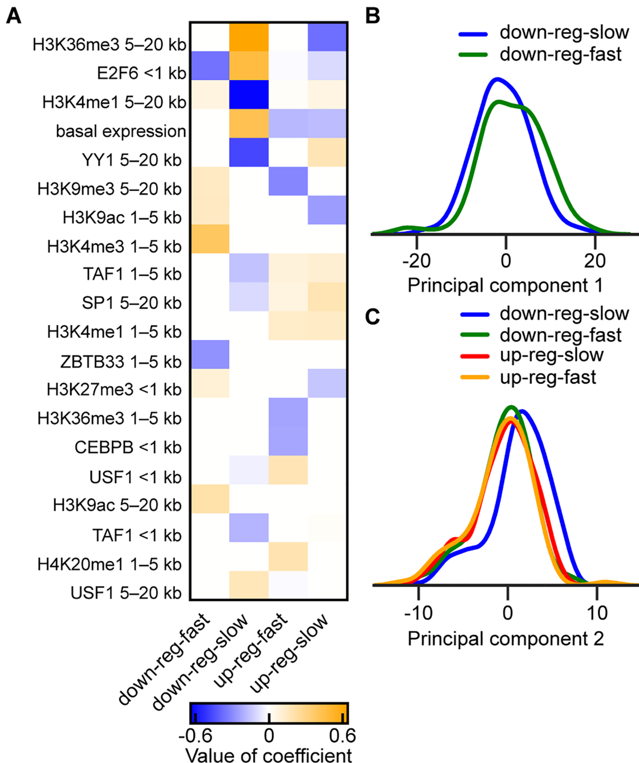
Fig 4. Differences in TF binding and histone modification occupancy in A549 cells in control conditions for the four largest DPGP clusters. (A) Heatmap shows the elastic net logistic regression coefficients for the top twenty predictors (sorted by sum of absolute value across clusters) of cluster membership for the four largest clusters. Predictors were \log_{10} library size-normalized binned counts of ChIP-seq TF binding and histone modification occupancy in control conditions. Distance indicated in row names represents the bin of the predictor (e.g., <1 kb means within 1 kb of the TSS). An additional 23 predictors with smaller but non-zero coefficients are shown in S6 Fig. (B) Kernel density histogram smoothed with a Gaussian kernel and Scott's bandwidth [63] of the TF binding and histone modification occupancy \log_{10} library size-normalized binned count matrix in control conditions
