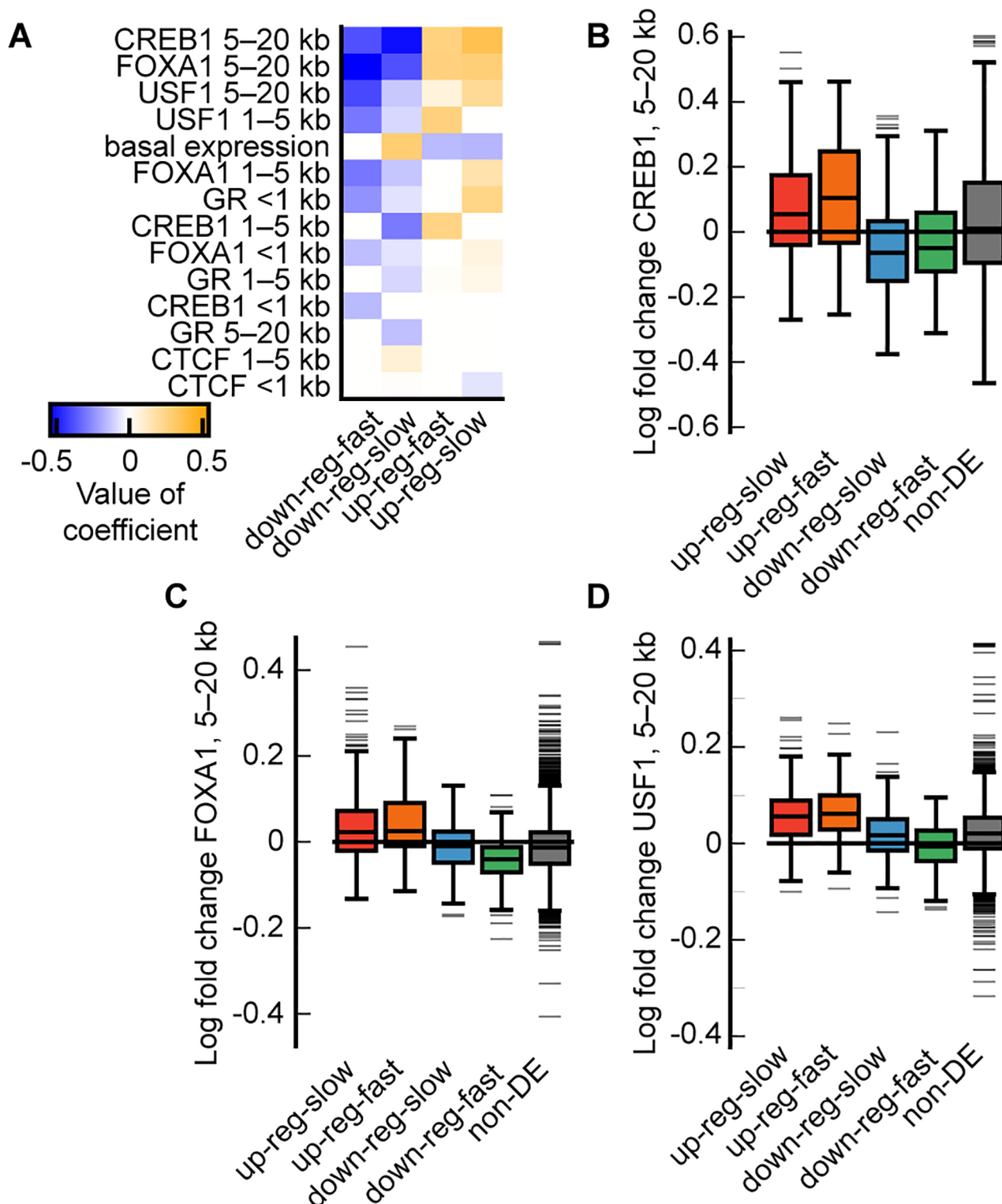
Fig 5. Differences in changes in transcription factor binding in A549 cells in response to glucocorticoid exposure for the four largest DPGP clusters. (A) Heatmap shows all coefficients (sorted by sum of absolute value across clusters) for predictors with non-zero coefficients as estimated by elastic net logistic regression of cluster membership for the four largest DPGP clusters. Predictors on y-axis represent log fold-change in normalized binned counts of TF binding from ethanol to dex conditions as assayed by ChIP-seq. Distance indicated in row names reflects the bin of the predictor (e.g., 1 kb = within 1 kb of TSS). (B) Boxplots show the logFC in normalized binned counts across clusters and for the group of non-DE transcripts for CREB1, (C) FOXA1, and (D) USF1.
