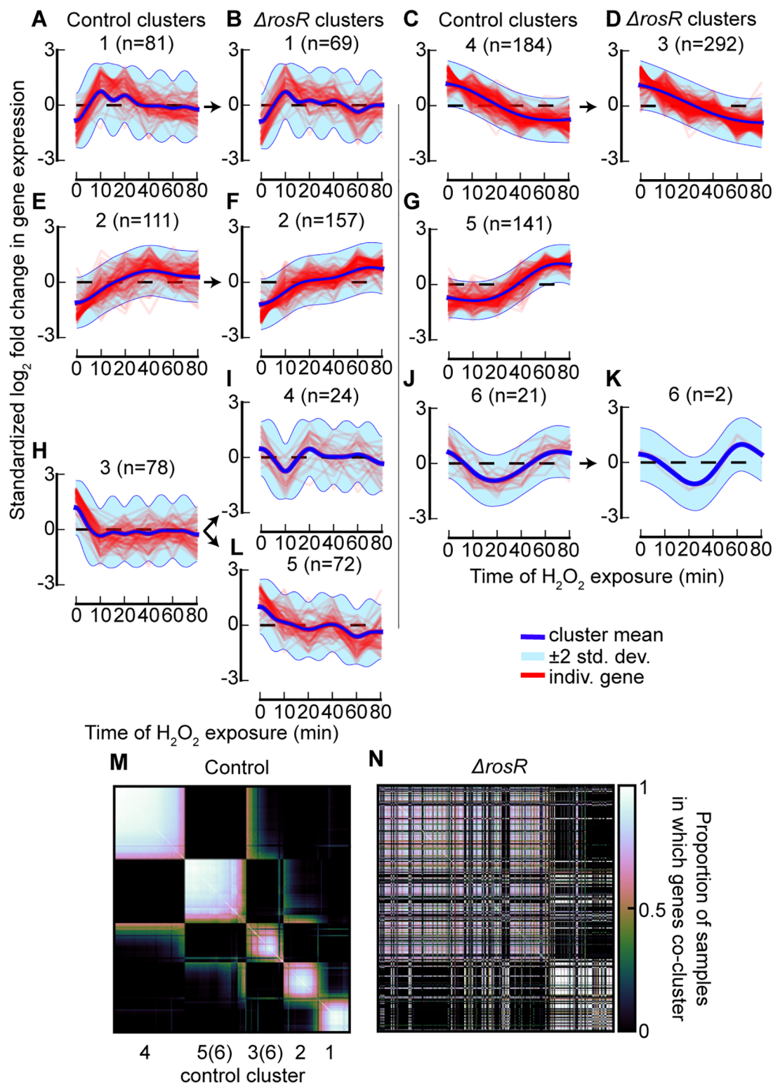
Fig 2. DPGP clusters in H. salinarum H_2O_2 -exposed gene expression trajectories. (A–L) For each cluster, standardized \log_2 fold change in expression from pre-exposure levels is shown for each gene as well as the posterior cluster mean \pm 2 standard deviations. Control strain clusters are on left and \Delta rosR clusters on right, organized to relate the \Delta rosR clusters that correspond to each control cluster. Note that control cluster 5 had no corresponding \Delta rosR cluster, but transcripts in this cluster instead distribute to a variety of \Delta rosR clusters, none of which had a majority of cluster 5 transcripts. (M) Heatmap displays the
