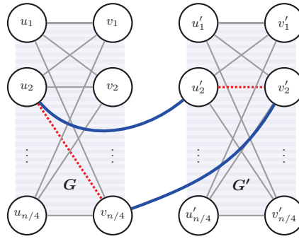
■ Figure 1 The lower bound graph B(G, G') for Theorem 9 with bridge edges (u_2, u'_2) and (v_{n/4}, v'_2) . The disconnected graph D is given by replacing the bridge edges with the dashed edges.
