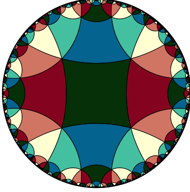
(a) Our colouring on the \{4, 6\} tiling in the Poincaré disk model.
