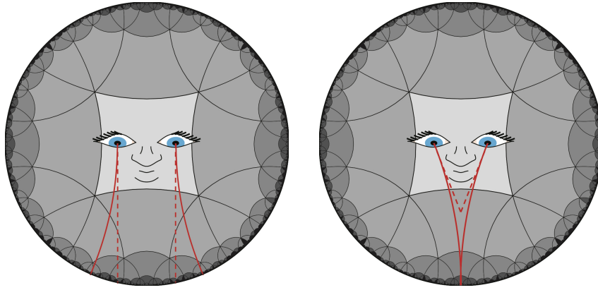
(a) Geodesics (light rays) from two eyes looking straight ahead would diverge in \mathbb{H}^2 . (b) Eyes must point inward to see an object that is infinitely far away in \mathbb{H}^2 .
