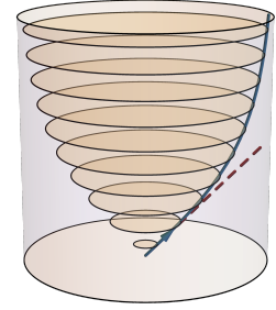
Figure 3: A geodesic in the (\text{Klein model}) \times \mathbb{E} (blue), and a straight line in \mathbb{E}^3 (red).
