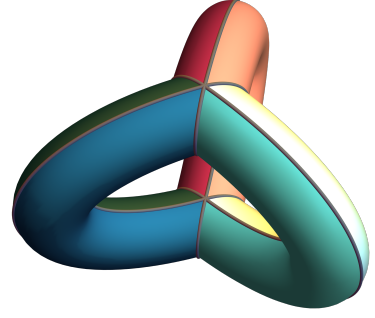
(c) The fundamental domain glued up to form a genus two surface.
