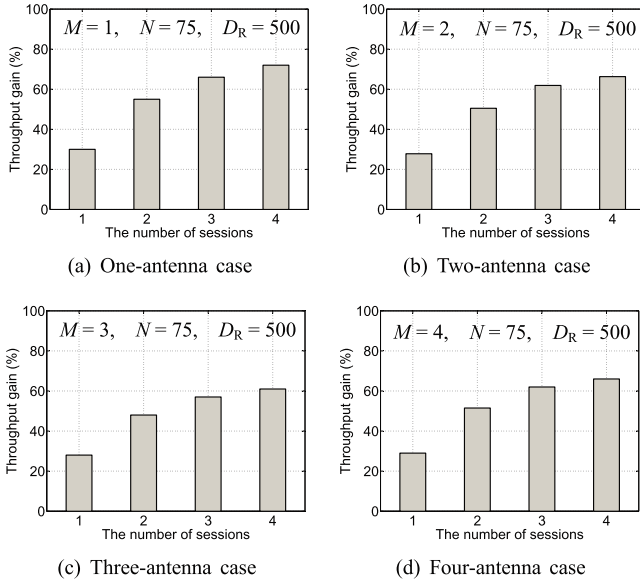
Fig. 9. The average throughput gain of IN versus the number of sessions, where M is the number of antennas, N is the total number of nodes, and D_R is the interference range.
