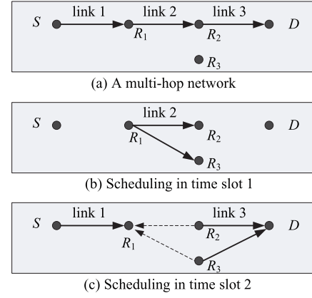
Fig. 1. An example that illustrates the benefits of IN in a three-hop network.
