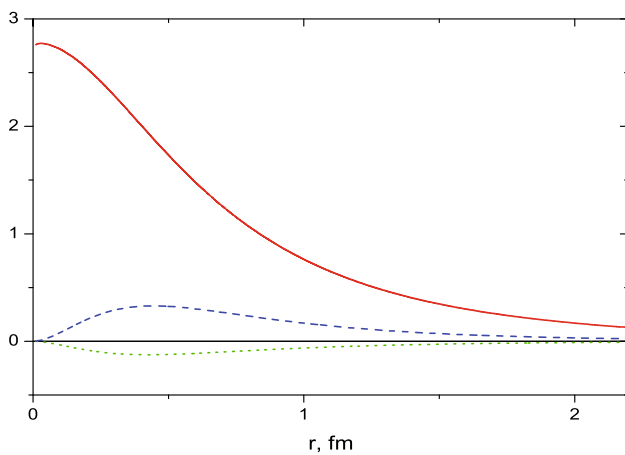
Fig. 1 Normalized wave functions of the \Sigma_c \bar{D}^* bound state with J^P = 3/2^- , T = 1/2 and the binding energy 14.6 MeV ( \Lambda = 1430 MeV). The |L = 0, S = 3/2\rangle , |L = 2, S = 1/2\rangle , and |L = 2, S = 3/2\rangle wave functions are solid, dotted, and dashed lines, respectively
