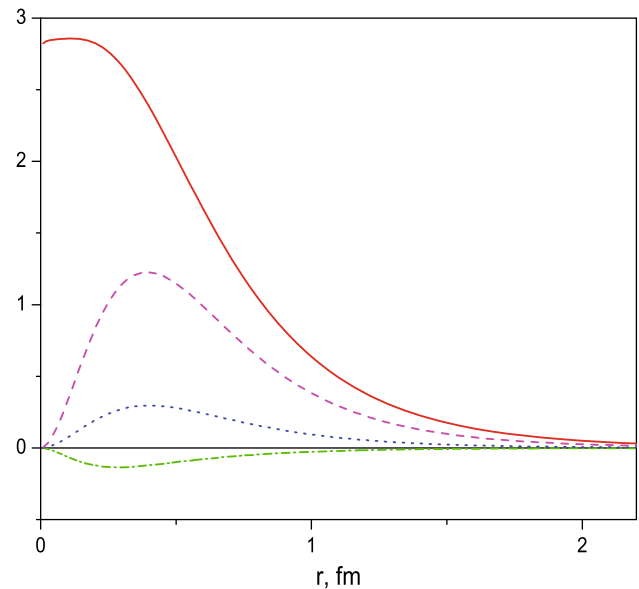
Fig. 2 Normalized wave functions of the \Sigma_c^* \bar{D}^* bound state with J^P = 5/2^-, T = 1/2 and the binding energy 74.8 MeV ( \Lambda = 1400 MeV). The |L = 0, S = 5/2\rangle , |L = 2, S = 1/2\rangle , |L = 2, S = 3/2\rangle , and |L = 2, S = 5/2\rangle wave functions are solid, dash-dotted, dotted, and dashed lines, respectively
