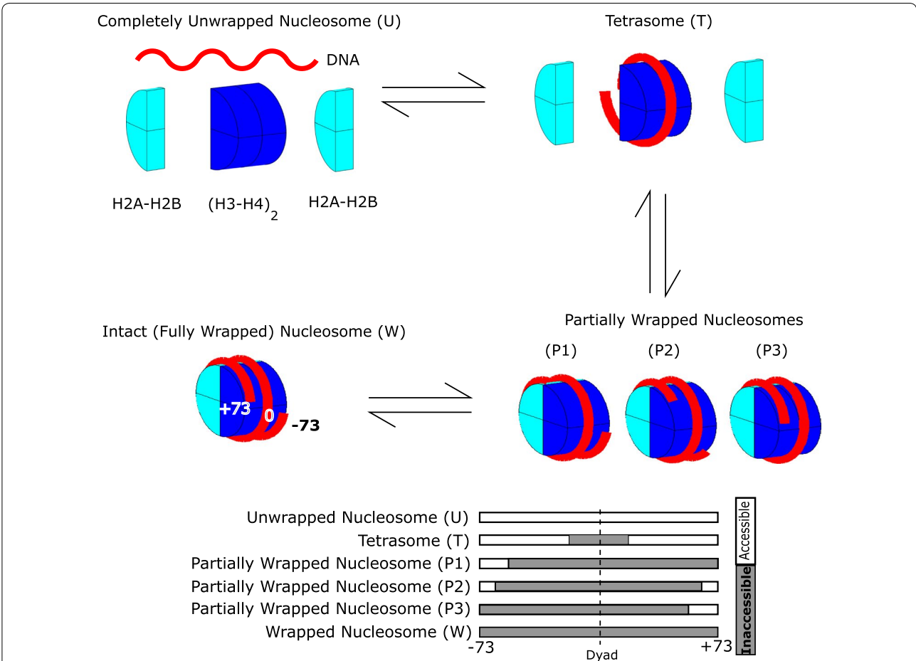
Fig. 1. The six conformational states used in the thermodynamic model of DNA accessibility in the nucleosome. The states differ by the degree of DNA accessibility and histone core composition. The DNA is completely inaccessible in the canonical nucleosome (W, wrapped). In each of the three partially wrapped conformations (P1, P3, P3) 20 bp are accessible. In the tetrasome (T), a total of 69 bp are accessible [62]. Each conformational state can also carry a post-translational modification (PTM) resulting in a total of twelve distinct energy states considered
