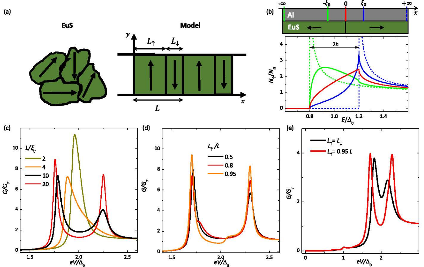
FIG. 4. Theoretical model of the tunneling conductance. (a) Sketches showing (left) the polycrystalline structure of the EuS and (right) the effective model of alternating up-down domains used in the simulation. We consider two lengths L_\uparrow and L_\downarrow and define L = L_\uparrow + L_\downarrow . The demagnetized phase is described by L_\uparrow = L_\downarrow , whereas after magnetization L_\uparrow \gg L_\downarrow . (b) Local density of states of the Aluminum on top of a two semi-infinite domain structure. The dashed lines show the spin-split BCS DoS deep inside the domains at x \rightarrow -\infty (blue) and x \rightarrow +\infty (green). By approaching the domain wall the DoS changes. Line traces of the plot the solid lines are taken at x = -\xi_0 (blue), x = 0 (red), and x = \xi_0 (green). (c) Averaged tunneling conductance calculated for an infinite stripe of balanced up/down domains L_\uparrow = L_\downarrow then describing the demagnetized EuS calculated for different domain size ( L ), \Gamma = 0.01 \Delta and T = 0.01 T_c . (d) Evolution of the tunneling conductance calculated at different magnetizations L_\uparrow and L = 10\xi_0 , \Gamma = 0.01 \Delta , and T = 0.01 T_c . (e) Tunneling conductance calculated for a demagnetized phase, made of six different domains, (black plot) and for a fully magnetized phase (red plot) including magnetic scattering.
