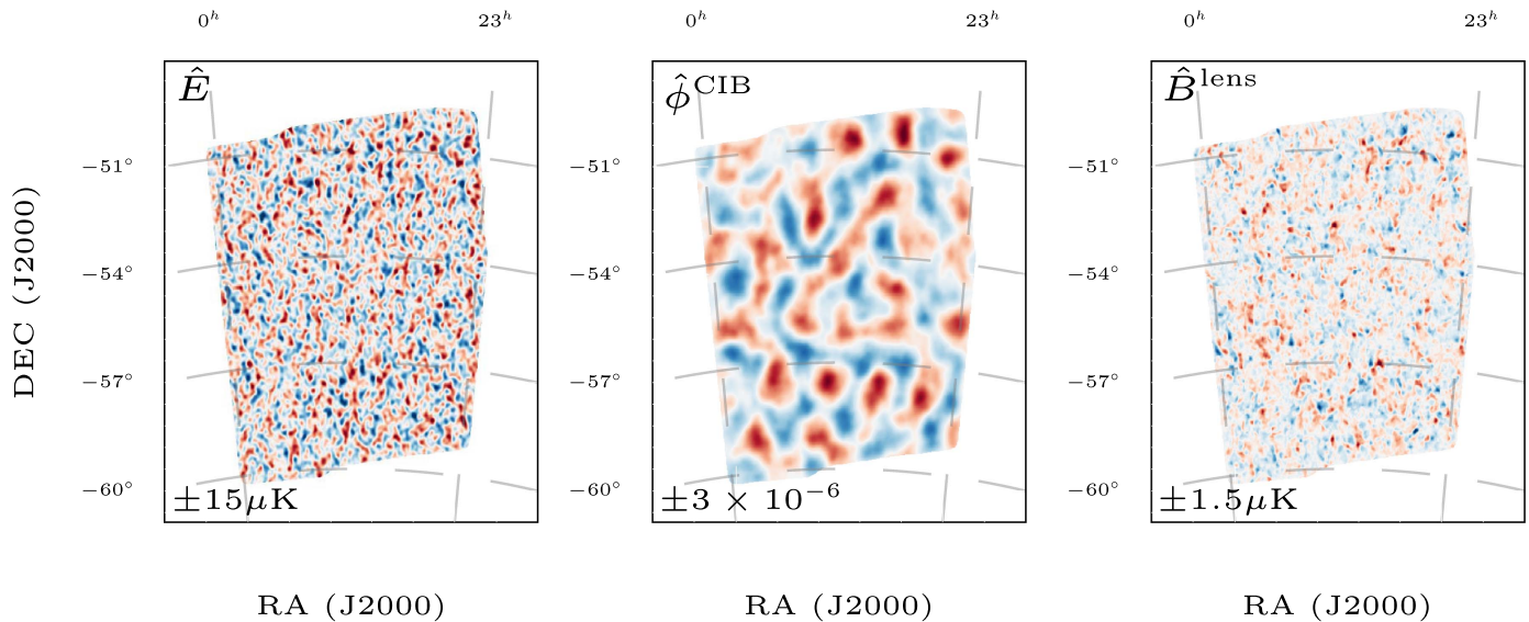
Figure 2. Maps used for delensing the data. The filtered E -mode map \bar{E}_\ell^{150} (left) is combined with a tracer of the CMB lensing potential obtained from filtering the CIB \hat{\phi}_\ell^{\text{CIB}} (center) in Fourier space to obtain a template of the lensing B modes \hat{B}_\ell^{\text{lens}} (right). This template is then subtracted from the B -mode data.
