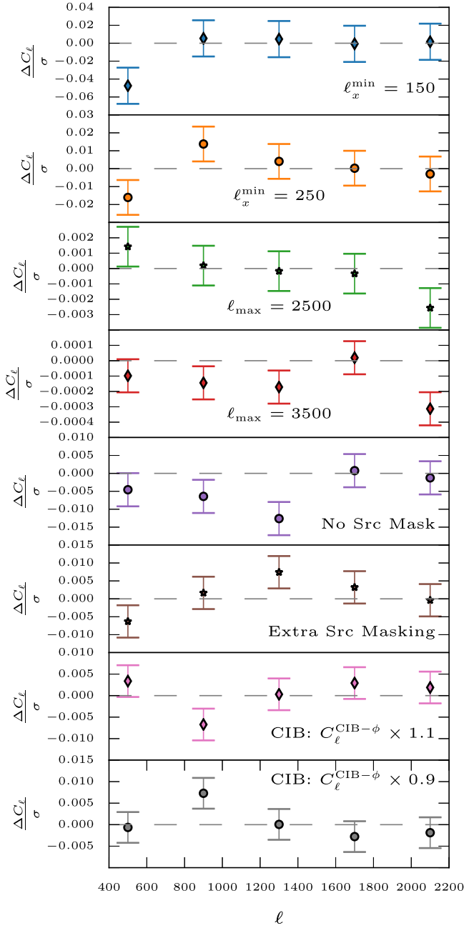
Figure 8. Systematic tests: the spectrum difference \Delta C_{\ell}^{\text{del}}_{b,\text{sys,data}} for each of the changes to the B -mode template described in Section 7.1, divided by the 1\sigma statistical uncertainty of the baseline delensed data spectrum ( C_{b,\text{data}}^{\text{del}} ). The error bars are calculated from the variance in simulations of each consistency test, i.e., the variance of (\Delta C_{b,\text{sys},i}^{\text{del}}) . We find the spectrum difference to be compatible with the changes observed in simulations, and small (less than 5%) compared to the statistical uncertainty.
