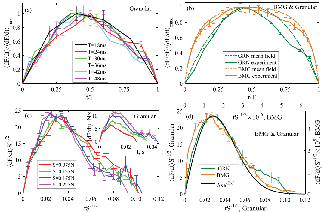
Figure 3. Temporal avalanche profiles in the universal scaling regime. (a) Average stress-drop rate normalized by the maximum rate of the granular system at the highest confining pressure. Profiles are averaged over avalanches from small bins of their durations. Error bars are calculated as standard error of the mean. (b) Stress-drop rates compared for metallic glass (brown) and granular material (green). Solid lines show averages over avalanches in the scaling regime. Dash-dotted curves show mean-field predictions with kT \approx 9 for the metallic glass data and kT \approx 0 for the granular data. (c) Granular stress-drop rates for fixed avalanche sizes S in the scaling regime ( S_{\min}^{\text{GRN}} < S < S_{\max}^{\text{GRN}} ). Inset shows original data, and main panel shows collapsed profiles scaled along both axes by S^{-1/2} . (d) Comparison of the averaged collapsed profiles for granular data (c) and metallic glass data 19 . The black curve shows scaling functions predicted by the mean-field model for both granular materials (bottom axis) and metallic glasses (top axis), which perfectly overlap with each other, further corroborating the similarity of the slip avalanche statistics of metallic glasses and granular materials. The granular fitting constants for the scaling function A \exp(-Bx^2) are A = 1.46 and B = 6.6 \times 10^{-4} ; the metallic glass constants are A = 3.98 \times 10^{11} and B = 2.18 \times 10^{11} .
