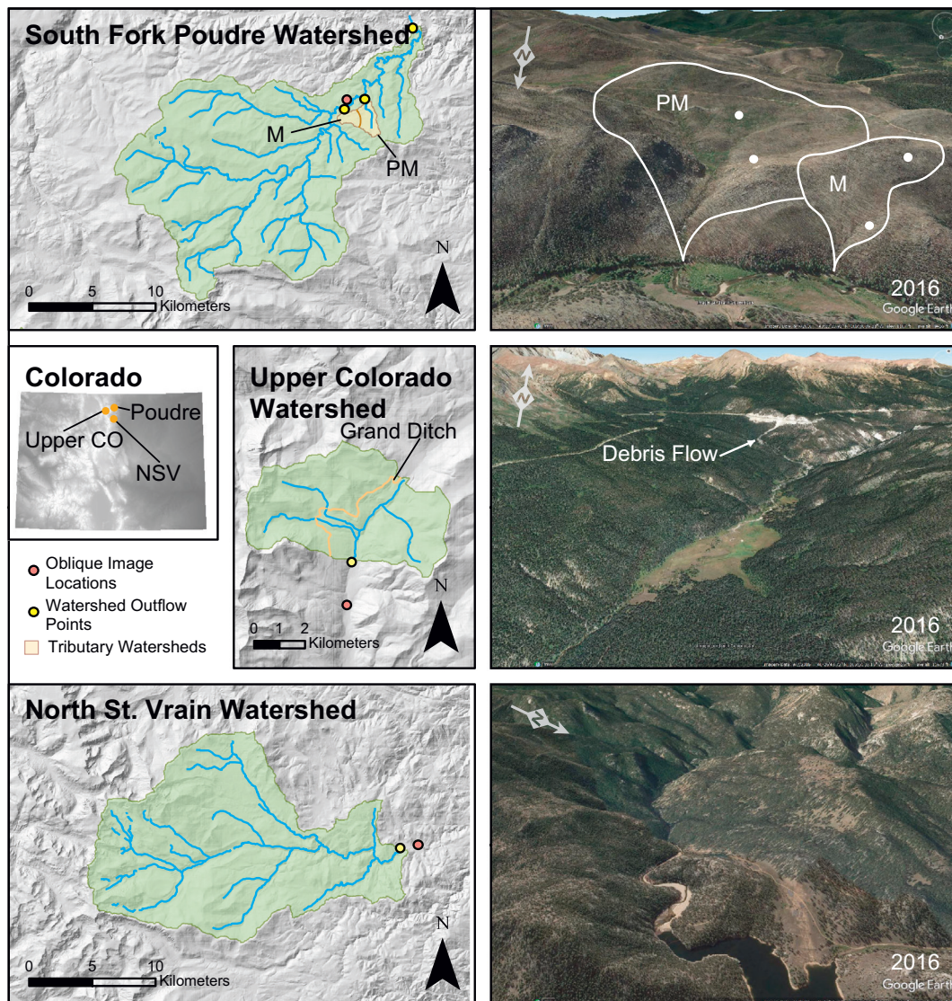
Fig. 1. Study watersheds in northern Colorado where sediment disturbances occurred between 2003 and 2013. A mulched (M) and partially mulched (PM) watershed within the South Fork Cache la Poudre basin was affected by the 2012 High Park fire and the 2013 Front Range flood. The white dots on the Google Earth image are locations of rain gages. The upper Colorado River received debris flow deposition from a breach in Grand Ditch in 2003. A 15-km study reach upstream from Ralph Price Reservoir along North St. Vrain Creek is where 2013 flood-related sediment erosion and deposition was particularly high. Evidence of that deposition (as light colored sediment) is captured in the Google Earth image at the inlet of the reservoir. Oblique Google Earth view is upstream on all images.
