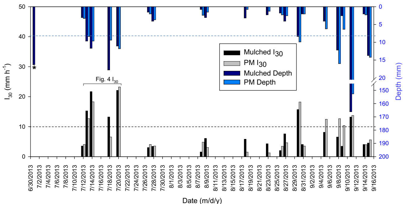
Fig. 3. Rainfall in 2013 as a maximum intensity 30-minute storm ( I_{30} ) and rainfall depth for mulched and partially mulched (PM) watersheds in the 2012 High Park fire burn area. Access to the field site to install instrumentation was not possible until June 2013. The 2013 September storms produced a >200-year event and widespread flooding throughout the Colorado Front Range. * indicates rainstorm totals measured prior to field instrumentation (E. Berryman unpubl. data), and the bracketed rainstorms from 13 to 20 Jul 2013 are shown in Fig. 4 with associated scour chain-derived sediment yields. Dashed lines are thresholds associated with erosion in other burned basins (Schmeer, 2014; Kampf et al., 2016). Rainfall intensity and depth in 2014 (not shown) produced just two storms (12 and 29 Jul 2014) that exceeded the 10 mm h -1 threshold for hillslope sediment production.
