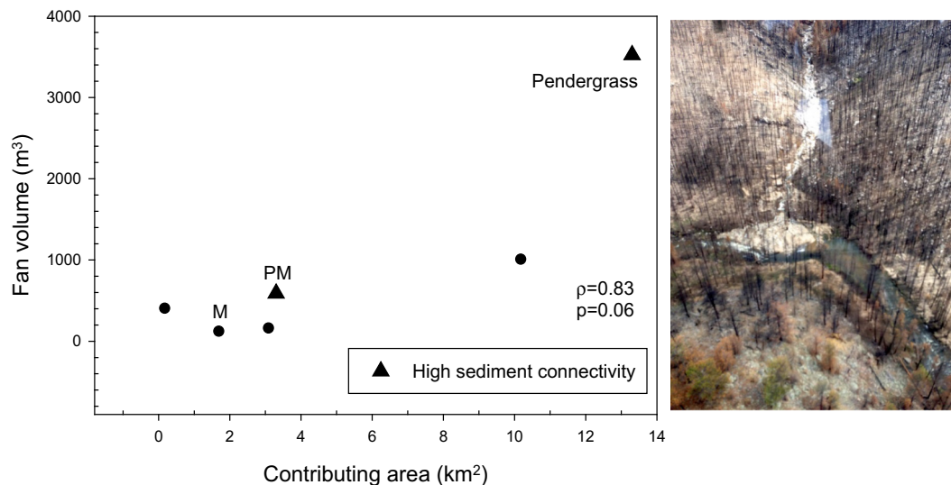
Fig. 6. Debris fan volume versus contributing area for six small watersheds within the South Fork Cache la Poudre basin. M indicates the mulched watershed and PM indicates the partially mulched watershed with all others not mulched. The Spearman correlation coefficient ( \rho = 0.83 ; p -value = 0.06) indicates a positive correlation between contributing area and fan volume with high connectivity influencing fan volume at two sites. Photo is of the fan at the confluence of Pendergrass Creek with the South Fork, 13 May 2013 (courtesy of B. Piehl). Flow is from right to left on the South Fork River.
