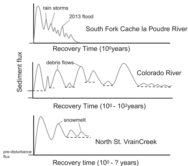
Fig. 8. Conceptual sediment recovery curves for the South Fork Cache la Poudre River, upper Colorado River (modified from Rathburn et al., 2013), and North St. Vrain Creek, northern Colorado. Relative sediment flux refers to discharge (mass per unit time) of sediment transported downstream following a disturbance. Sediment flux begins at conditions that existed prior to the disturbance. For the Colorado River, the short horizontal bar on the y-axis demarcates elevated starting sediment loads from anthropogenic influences of Grand Ditch, and logging and mining activities in the valley (Rubin et al., 2012; Rathburn et al., 2013; Grimsley et al., 2016). Likewise, the horizontal dashed lines within each plot indicate a shifting baseline of sediment recovery as a result of the increased frequency of disturbances or because of a new system state associated with the presence of an impounding reservoir, such as on North St. Vrain Creek.
