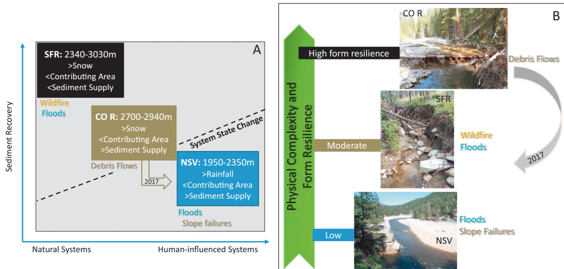
Fig. 9. (A) Sediment recovery for case studies along a natural to human-influenced gradient. Sediment recovery may not reflect channel form resilience because of a lack of physical complexity (B). While the upper Colorado River (CO R) shows moderate sediment recovery (A), high form resilience caused by channel-spanning log steps creates bedforms and habitat. The form complexity and resilience is downgraded because of another debris flow in summer 2017 (downward arrows in A and B). The South Fork River (SFR) and North St. Vrain (NSV) have lower form resilience owing to incised channels without the physical channel complexity (B).
