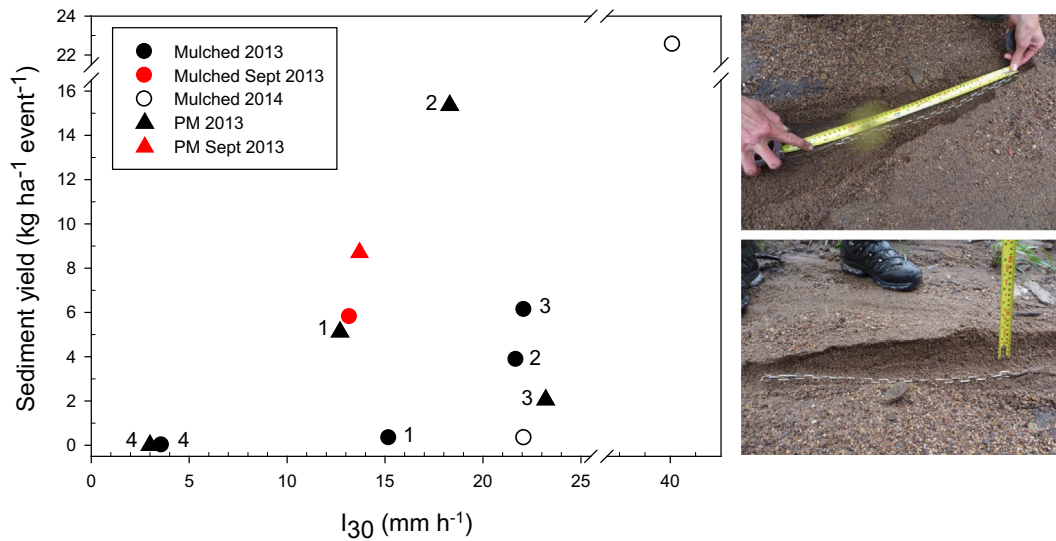
Fig. 4. Sediment yield versus maximum intensity 30-minute storm ( I_{30} ) for ephemeral channels within the mulched and partially mulched (PM) watersheds in the South Fork Cache la Poudre basin. Photos show scour chains installed in the bed at channel cross sections on first order streams in the mulched watershed (location shown in left photo of Fig. 2) that were used to estimate event sediment yields, assuming a 1-m reach length and unit channel width. Numbers adjacent to symbols indicate common rain storms between the mulched and partially mulched watersheds as follows: 1 = 13 Jul 2013; 2 = 14 Jul 2013; 3 = 20 Jul 2013; 4 = 28 Jul 2013. Data are missing for 2014 for the PM basin because the scour chains were eroded out and lost. (Photos courtesy of M. Dixon.)
