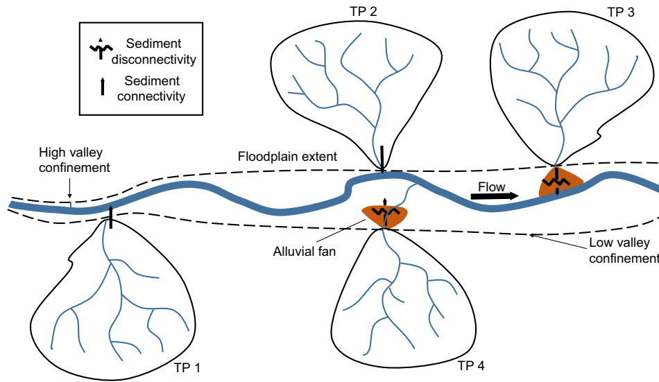
Fig. 11. Sediment connectivity and disconnectivity influences on post-fire treatment priorities. TP1–TP4 represents watersheds with highest (TP1) to lowest (TP4) treatment priority based on sediment connectivity. In the South Fork River paired watersheds, the mulched watershed represents TP4 because of the wider floodplain and development of a sediment fan, whereas the partially mulched watershed represents TP1 with high valley confinement and high sediment connectivity.
