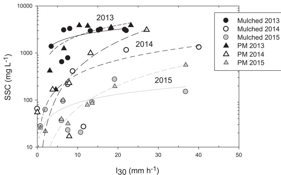
Fig. 5. Peak suspended sediment concentration (SSC) associated with maximum intensity 30-minute storm ( I_{30} ) measured at the outlets of the mulched and partially mulched (PM) watersheds tributary to the South Fork River. Maximum SSC in 1989 and 1997 (pre-fire background levels) from a site 4 km upstream is 100 \text{ mg L}^{-1} . SSC had largely recovered to background levels by 3 years post-fire in the mulched and in the partially mulched watersheds. The 2014 data includes residual impacts of the September 2013 flood as well as rain storms during that year.
