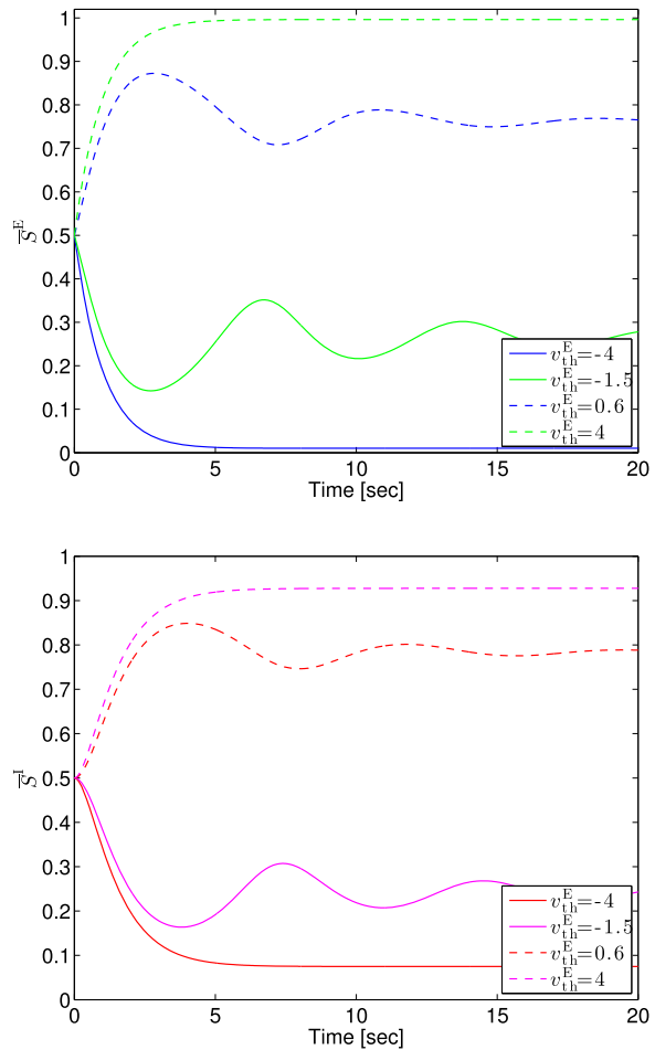
Fig. 7 Mean synaptic drives for a = 10, b = 9, c = 6, d = 1, v_{th}^I = -2.5, \lambda^E = 1, \lambda^I = 1, f_{max} = 1 , and \gamma = 1 with \bar{S}^E(0) = 0.5 and \bar{S}^I(0) = 0.5 and with different values of v_{th}^E
