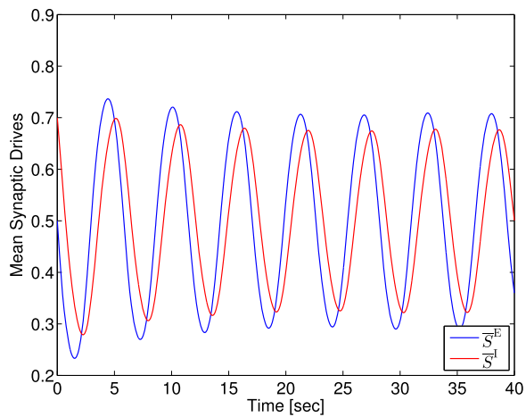
Fig. 3 \bar{S}^E(t) and \bar{S}^I(t) versus time for a = 10 , b = 9 , c = 6 , d = 1 , v_{th}^E = -0.5 , v_{th}^I = -2.5 , \lambda^E = 1 , \lambda^I = 1 , f_{max} = 1 , and \gamma = 1 with \bar{S}^E(0) = 0.5 and \bar{S}^I(0) = 0.7
