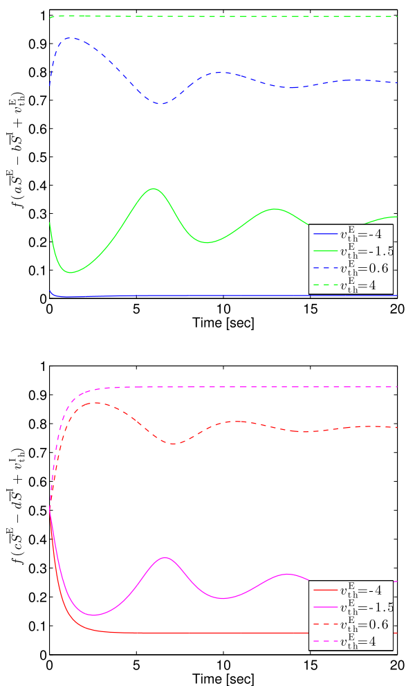
Fig. 6 Mean firing rates for a = 10 , b = 9 , c = 6 , d = 1 , v_{th}^I = -2.5 , \lambda^E = 1 , \lambda^I = 1 , f_{max} = 1 , and \gamma = 1 with \bar{S}^E(0) = 0.5 and \bar{S}^I(0) = 0.5 and with different values of v_{th}^E
