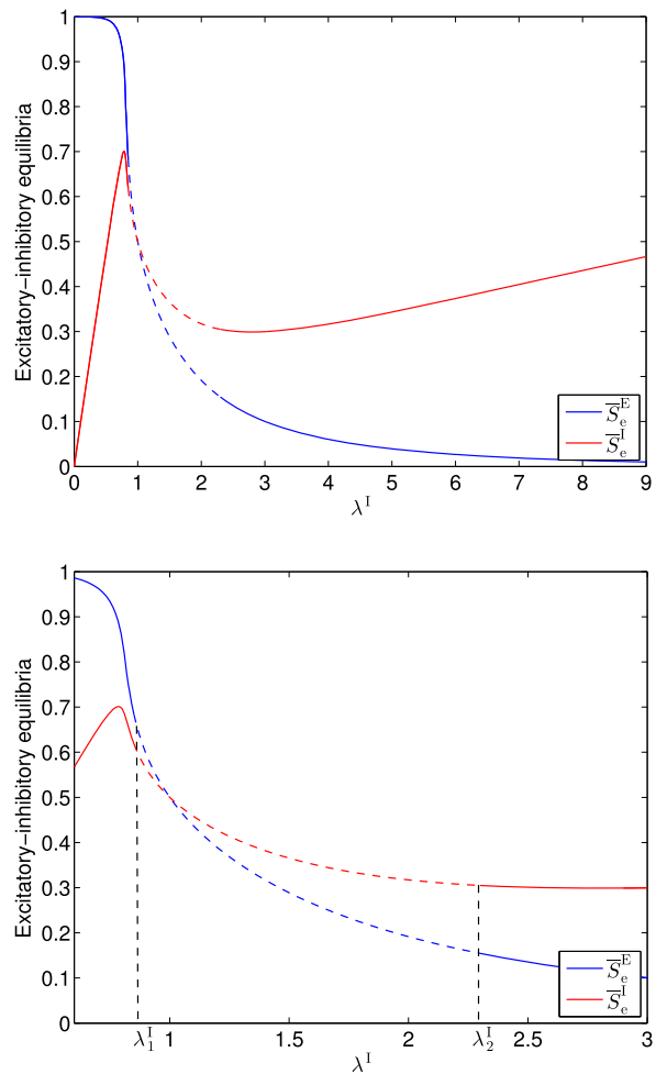
Fig. 9 Bifurcation diagram of (11) and (12) for a = 10 , b = 9 , c = 6 , d = 1 , v_{th}^E = -0.5 , v_{th}^I = -2.5 , \lambda^E = 1 , f_{max} = 1 , and \gamma = 1 with \lambda^I as a bifurcation parameter. The solid line represents asymptotically stable equilibrium point, whereas the dashed line represents unstable equilibrium point. A supercritical Hopf bifurcation occurs at \lambda_1^I = 0.85 where the single asymptotically stable equilibrium point becomes unstable and gives rise to a stable limit cycle. At \lambda_2^I = 2.3 , the unstable equilibrium point reverts to an asymptotically stable equilibrium point and the stable limit cycle disappears
