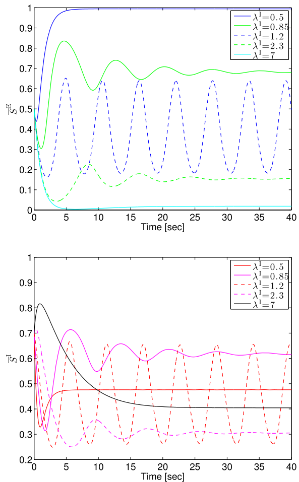
Fig. 10 Mean synaptic drives for a = 10 , b = 9 , c = 6 , d = 1 , v_{th}^E = -0.5 , v_{th}^I = -2.5 , \lambda^E = 1 , f_{max} = 1 , and \gamma = 1 with \bar{S}^E(0) = 0.5 and \bar{S}^I(0) = 0.7 and with different values of \lambda^I
