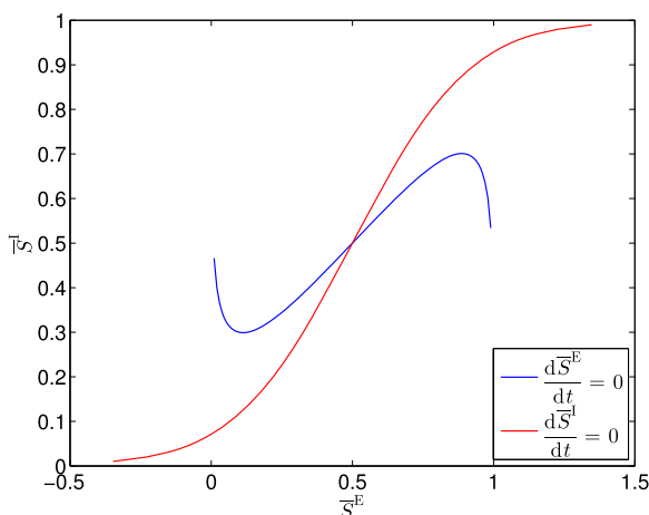
Fig. 2 Plots of \frac{d\bar{S}^E}{dr} = 0 and \frac{d\bar{S}^I}{dr} = 0 for a = 10 , b = 9 , c = 6 , d = 1 , v_{th}^E = -0.5 , v_{th}^I = -2.5 , \lambda^E = 1 , \lambda^I = 1 , f_{max} = 1 , and \gamma = 1
