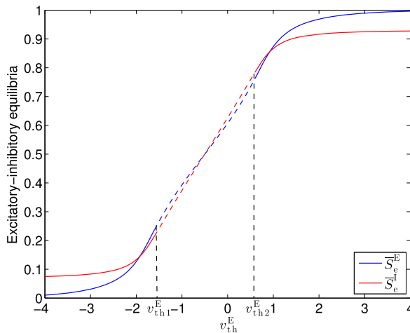
Fig. 5 Bifurcation diagram of (11) and (12) for a = 10 , b = 9 , c = 6 , d = 1 , v_{th}^I = -2.5 , \lambda^E = 1 , \lambda^I = 1 , f_{max} = 1 , and \gamma = 1 with v_{th}^E as a bifurcation parameter. The solid line represents asymptotically stable equilibrium point, whereas the dashed line represents unstable equilibrium point. A supercritical Hopf bifurcation occurs at v_{th}^E = -1.6 where the single asymptotically stable equilibrium point becomes unstable and gives rise to a stable limit cycle. At v_{th}^E = 0.6 , the unstable equilibrium point reverts to an asymptotically stable equilibrium point and the stable limit cycle disappears
