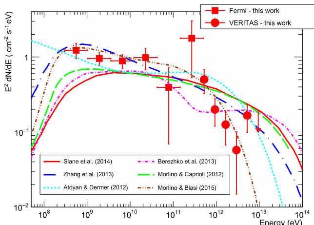
Figure 5. Fermi and VERITAS SEDs with theoretical models. Filled red squares show the Fermi results and filled red circles show the VERITAS results from this study. The models discussed in the text appear as the solid red line (preferred model A from Slane et al. 2014), the magenta short broken dashed line (Bereztko et al. 2013), the blue large broken dashed line (Zhang et al. 2013), the green dashed line (Morlino & Caprioli 2012), the cyan dotted line (the leptonic model from Atoyan & Dermer 2012), and the brown double-broken dashed line (Morlino & Blasi 2016, with a neutral fraction of 0.6). The data used to create this figure are available.
