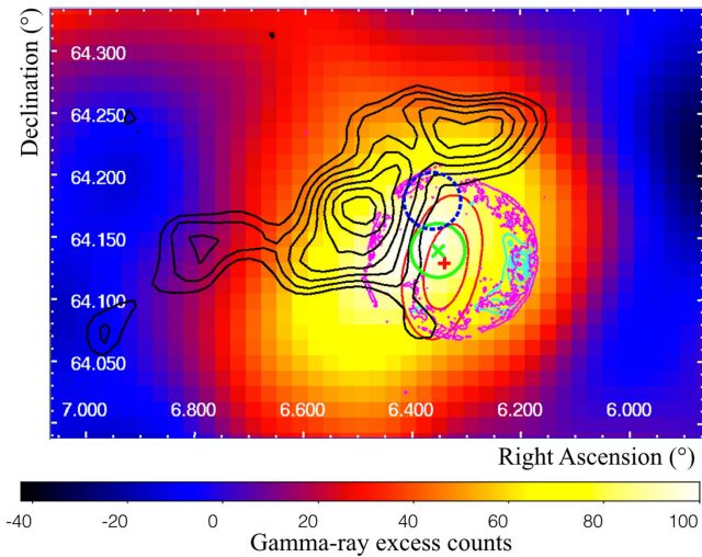
Figure 3. Smoothed VERITAS gamma-ray count map of the region around Tycho’s SNR. The 1\sigma statistical error on the centroid position obtained by Acciari et al. (2011) is drawn with a blue dashed circle. The updated centroid position is marked with a red cross, and the 68% and 95% confidence levels of the position are shown with red contours. Each contour was determined from a fit with two degrees of freedom. Chandra ’s measurement of the X-ray emission with energies larger than 4.1 keV is shown by the magenta contours. Black contours are the ^{12}\text{CO} ( J = 1-0 ) emission integrated over the velocity range -68 \text{ km s}^{-1} to -50 \text{ km s}^{-1} using the measurements from the Five College Radio Astronomy Observatory Survey (Heyer et al. 1998). NuSTAR ’s measurements of X-rays in the energy range between 20 keV and 40 keV (Lopez et al. 2015) after smoothing are shown by the cyan contours. The best-fit position and 68% confidence level of the updated Fermi analysis are shown as a green x mark and circle.
