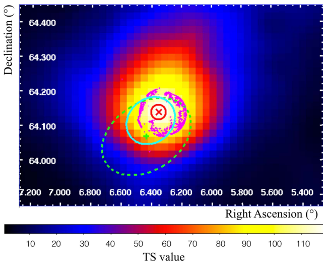
Figure 1. Smoothed Fermi TS map with the P8R2_CLEAN_V6 IRF for energies higher than 1 GeV. The map was smoothed with a Gaussian kernel with a radius of 0^{\circ}06 . The magenta contours indicate the Chandra X-ray intensity at energies above 4.1 keV ( http://chandra.harvard.edu ). The cyan line is the previously published 95% confidence area for the Fermi -LAT position (Giordano et al. 2012). The centroid and error of 3FGL J0025.7+6404 are marked with a cross and dashed green line (Acero et al. 2015). The best-fit position and 68% confidence level of this study are shown with a red cross mark and a red circle.
