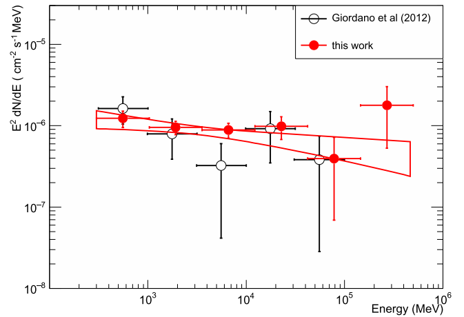
Figure 2. Updated Fermi spectrum overlaid with the previous results. The solid red line shows the 1\sigma statistical error band from the full fit.
