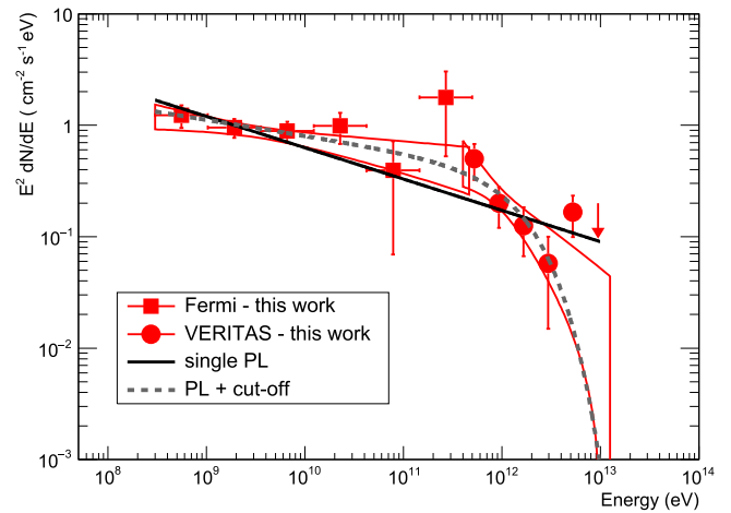
Figure 6. Fermi and VERITAS SEDs overlaid with the combined fit results. Flux errors calculated from the error propagation of the fitting function are drawn as a 1\sigma statistical error band in red lines. The Fermi –VERITAS combined fit results with a single power-law fit and a single power law with a cutoff are shown with a black solid line and a gray short dashed line.
