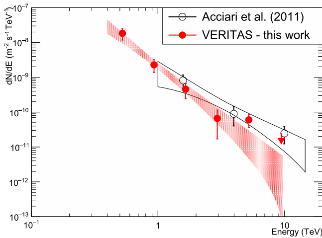
Figure 4. VERITAS spectra. The previous result is plotted as black empty circles, and the result of the present study is shown with filled red circles. Flux errors were calculated from error propagation of the fitting function and drawn as a 1\sigma error band around the data points.
