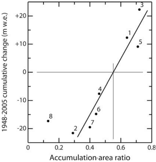
Fig. 6. 1948–2005 cumulative change of eight reconstructed–observed b_n series vs accumulation-area ratio (AAR). The straight line, which has \text{rms} = 4.3 \text{ m w.e.} , is fit to only points 1–7. See Table 1 for glacier names.
