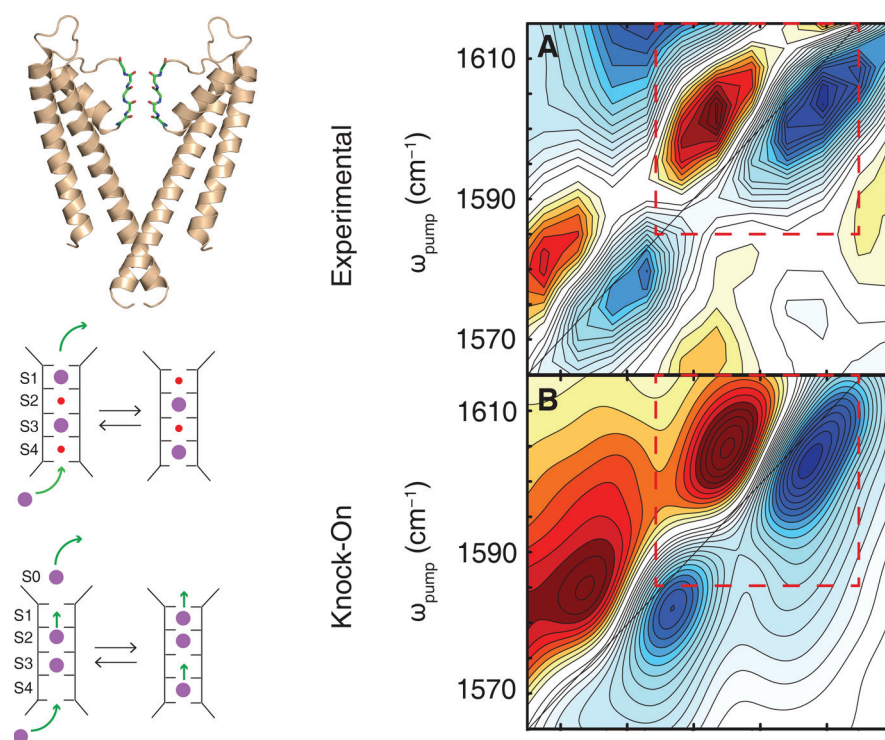
Figure 3. Left: The KcsA potassium ion channel and a schematic of the knock-on (top) and hard-knock (bottom) ion transport mechanisms. Right: (a) The experimental IR spectrum in the isotope labeled region and (b) the simulated 2D IR spectrum of the knock-on model. Reproduced with permission from refs 4 and 74. Copyright 2017 American Chemical Society and 2016 American Association for the Advancement of Science, respectively.
