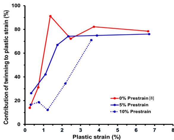
Fig. 8. Contribution of \{10\bar{1}2\} extension twinning to plastic strain at the low stress stage for 0%, 5% and 10% prestrain. At plastic strains < 1.0\% , the contribution of twinning is relatively insignificant, especially for the 10% prestrained specimen in which a plateau is present when \epsilon_p < 1.2\% . In general, prestrains push the curves to the right. 5% prestrain slightly reduces the contribution of twinning to plastic strain at low strains. However, 10% prestrain significantly reduces the contribution when \epsilon_p < 3.5\% , indicating retardation of twinning at low strains.
