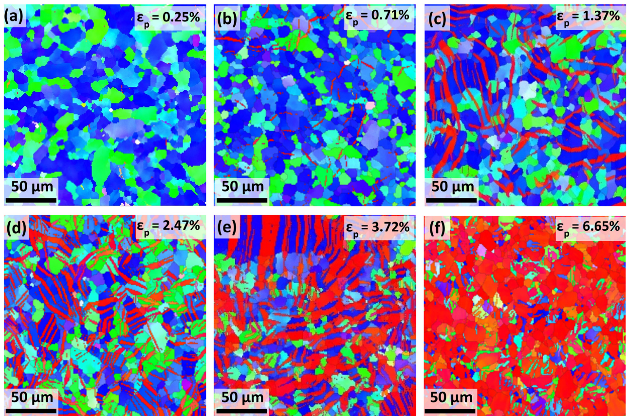
Fig. 4. IPF maps at selected plastic strain levels for 0% prestrain (monotonic compression).
