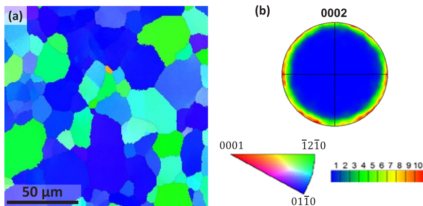
Fig. 1. Initial grain structure and texture of the as-extruded AZ31 alloy. The scanned surface is perpendicular to the extrusion direction (ED). (a) Inverse pole figure (IPF) map. (b) Pole figure. The basal planes are mostly parallel to the ED, which is a typical of extruded Mg alloys.
