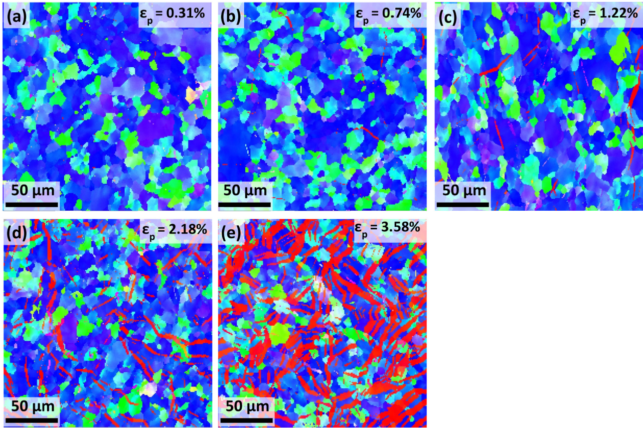
Fig. 6. IPF maps at selected plastic strain levels for the specimen with 10% prestrain. Compared with 0% and 5% prestrains, the number of twins is much lower at the early stage when \epsilon_p < 2.18\% . Obviously, twin nucleation is retarded by prestrain.
