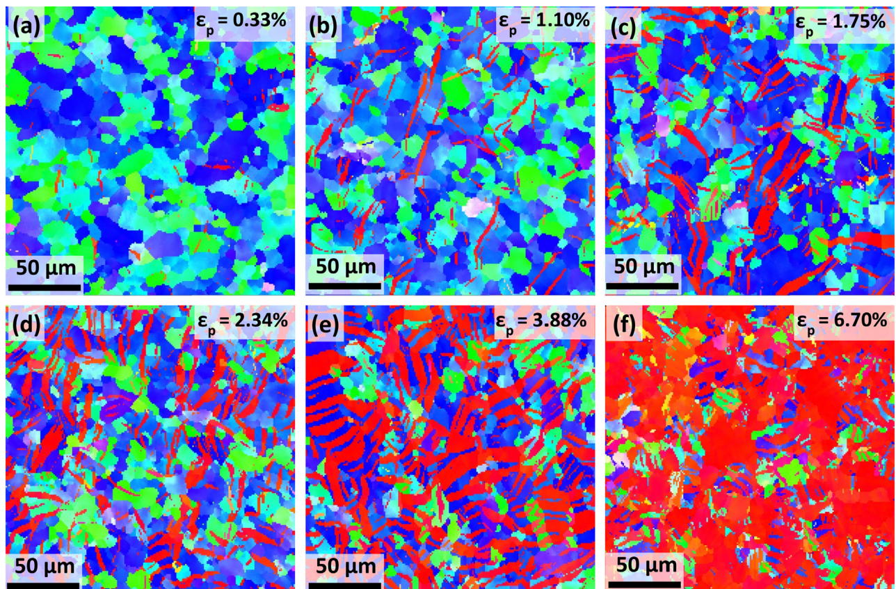
Fig. 5. IPF maps at selected plastic strain levels for the specimen with 5% prestrain. The twinning behavior is similar to the specimen without prestrain.
