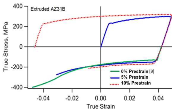
Fig. 3. Comparison of stress-strain curves for 0%, 5%, and 10% prestrains by overlapping the flow stages of three specimens. The yield stress under compression only slightly increases with increasing prestrain. However, the hardening rate at the low stress stage during compression remains practically unchanged [38].
