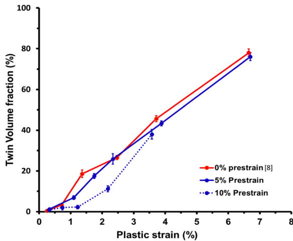
Fig. 7. Evolution of twin volume fraction (TVF, f_{twin} ) as a function of plastic strain. The TVFs for the different prestrains were measured from the IPF maps in Figs. 4–6, respectively. At least three measurements were performed at each plastic strain level and the averaged value was plotted. The TVF for 5% prestrain is close to the TVF without prestrain. However, at strains < 3.5\% , the TVF for 10% prestrain is lower than that for 0% and 5% prestrain.
