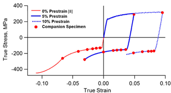
Fig. 2. Stress-strain curves with 0% pre-tension strain (red line), 5% pre-tension strain (blue solid line), and 10% pre-tension strain (blue dashed line). The red dots denote strain levels at which companion specimens were terminated for EBSD analysis [38].
