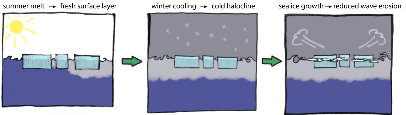
Fig. 4. Proposed mechanism for prolonged iceberg lifetimes. Left: summer melt of icebergs creates a shallow fresh surface layer. Middle: As temperatures drop during fall, the fresh surface layer remains lighter than the saltier waters below. Right: This allows for sea ice to grow as the temperature of the surface layer drops below freezing, which in turn protects the icebergs from wave-induced sidewall erosion and prolongs their lifetimes.
