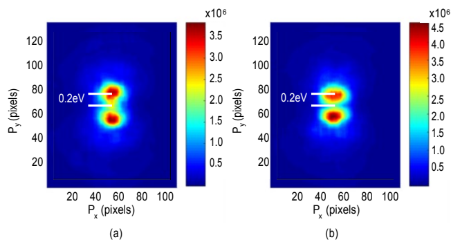
FIG. 5. Example 2D FFT VMI analysis images showing (a) X -state modulation and (b) A -state modulation. The pump and probe are vertically polarized 800-nm light. In addition to five-block averaging these images have also been smoothed to enhance the modulation signal. Also shown is the 0.2 eV radial distance consistent with dissociation through the B state. Note that since a slightly lower repeller voltage was used to magnify the (1,0) channel, these images have been scaled to the same image size as the single-pulse images used in this paper.
