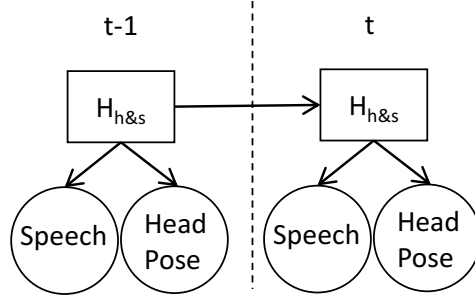
Figure 2. The diagram of the DBN proposed by Mariooryad and Busso [8]. We build the proposed models starting from this structure.
