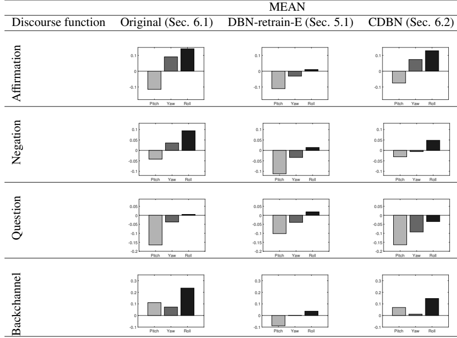
Figure 6. The average of head angles per discourse function for the original head motion (Sec. 6.1), and the synthesized sequences using DBN-retrain-E (Sec. 5.1) and CDBN (Sec. 6.2).
