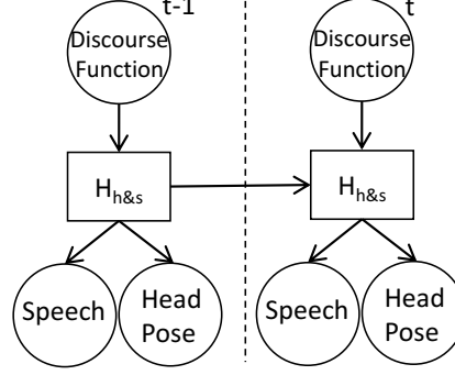
Figure 8. The constrained DBN (CDBN). It introduces explicit dependencies on the discourse functions, creating meaningful behaviors.
