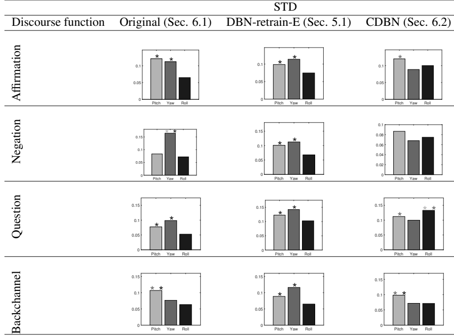
Figure 7. The average of the standard deviation for each discourse function for the original head movements (Sec. 6.1), and the synthesized sequences with DBN-retrain-E (Sec. 5.1) and CDBN (Sec. 6.2).
