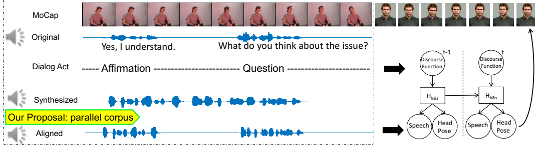
Figure 1. Overview of the proposed method.
