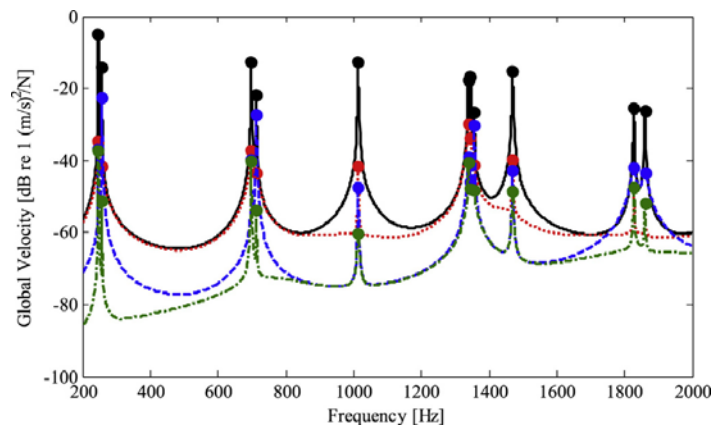
Fig. 13. Effect of active patch location on the predicted global mean-square velocity of shell, \Psi_{\text{g}}^2 , as compared to uncontrolled (—), where modal values are indicated by (•): (a) location 1 (•••); location 2 (•••); location 3 (•••).
