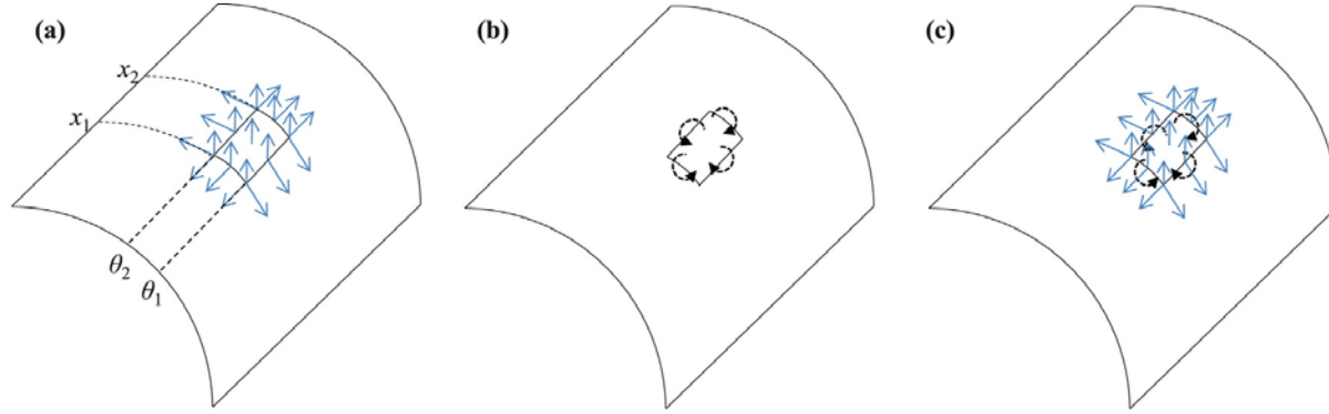
Fig. 4. Equivalent loading from alternate active patch configurations on a shell section: (a) in-phase bimorph with F_x , F_\theta , and P_r ( \rightarrow ) and patch endpoints labeled; (b) out-of-phase bimorph with M_x and M_\theta ( \rightarrow ); (c) proposed combined loading representation of unimorph.
