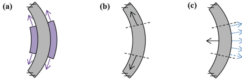
Fig. 3. Effective distributed pressure loading: (a) in-phase actuation; (b) equivalent force loading; (c) resultant of equivalent force ( \leftarrow ) needs to be balanced by an effective pressure ( \rightarrow ).
