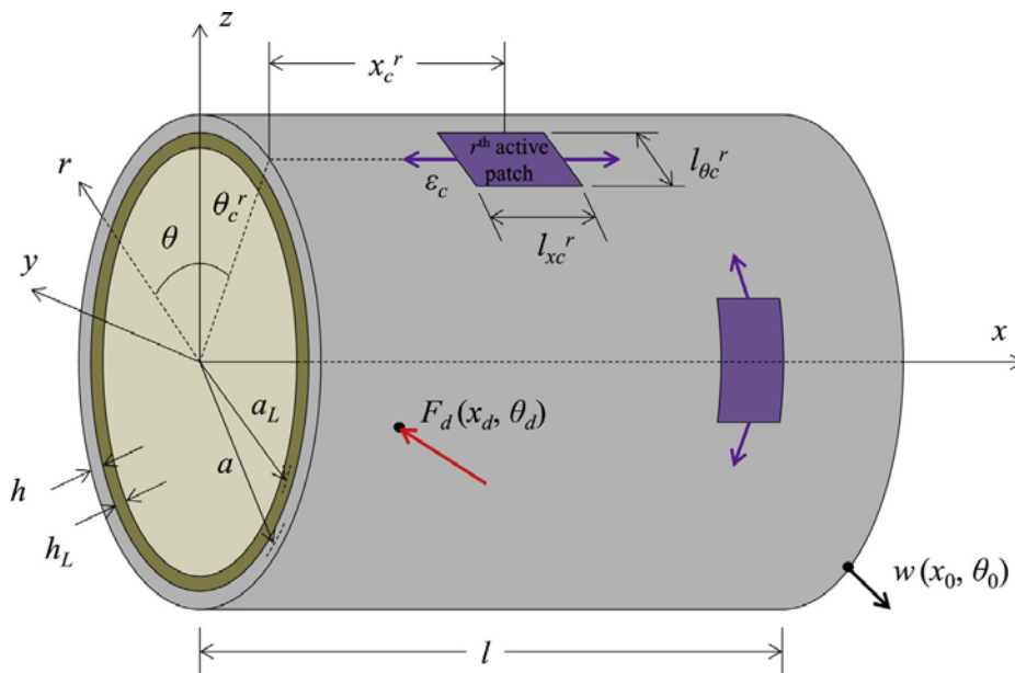
Fig. 1. Example case: active patches and cardboard liner on a thin cylindrical shell with free boundaries (extension of the system studied in [1]); patch size/ location and force/measurement location are labeled; see Nomenclature and text for definition of symbols.
