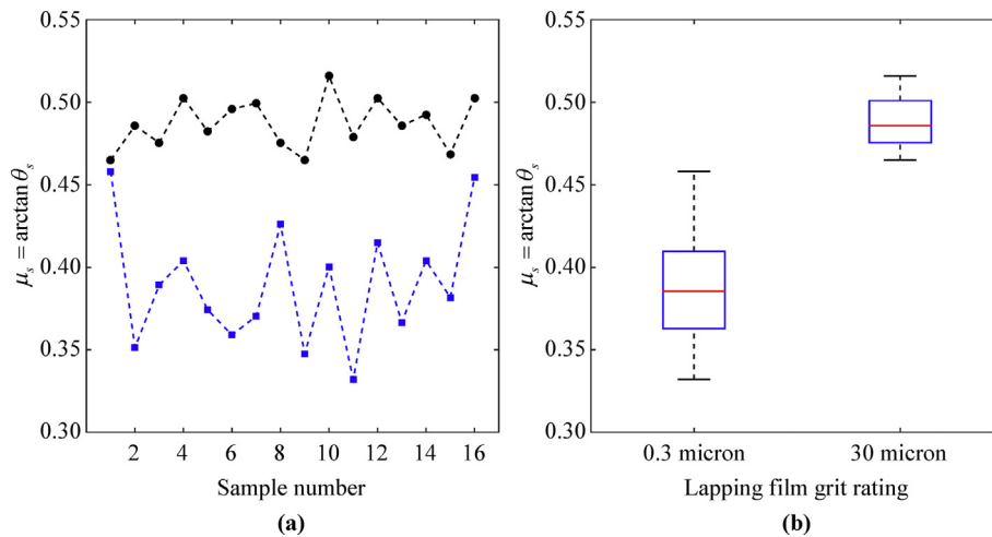
Fig. 5. Measured static friction values for 16 samples using the apparatus of Fig. 4. (a) \mu_s determined from each measured \theta_s , where \cdots\bullet\cdots are 30 \mu\text{m} lapping film points and \cdots\square\cdots are the 0.3 \mu\text{m} lapping film points. (b) Boxplot of experimentally determined \mu_s for each lapping film grit.
