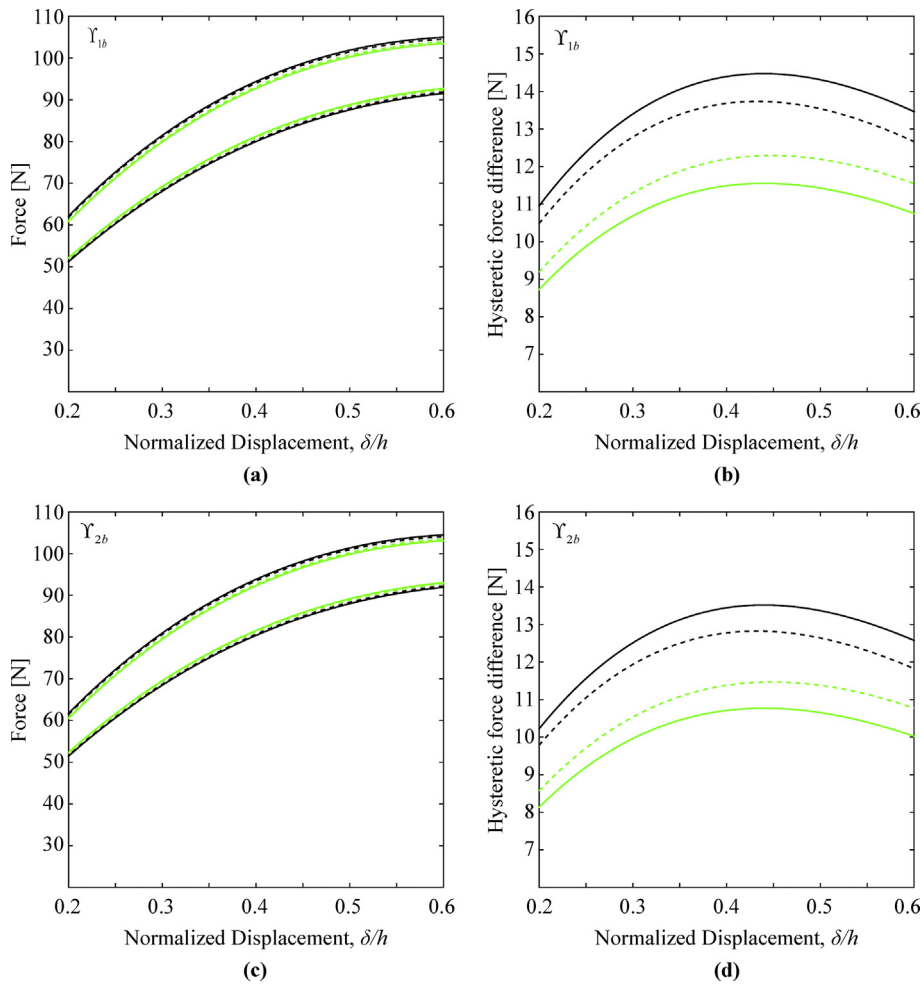
Fig. 12. Analytical results for refined models Y_{1b} and Y_{2b} ( c = b ) for the conditions described in Table 8. (a) Load-displacement curves for model Y_{1b} , (b) hysteretic force difference curves for model Y_{1b} , (c) load-displacement curves for model Y_{2b} , and (d) hysteretic force magnitude curves for model Y_{2b} . Key: — \Phi_1 , — \Phi_2 , --- \Phi_3 , and - - \Phi_4 .
