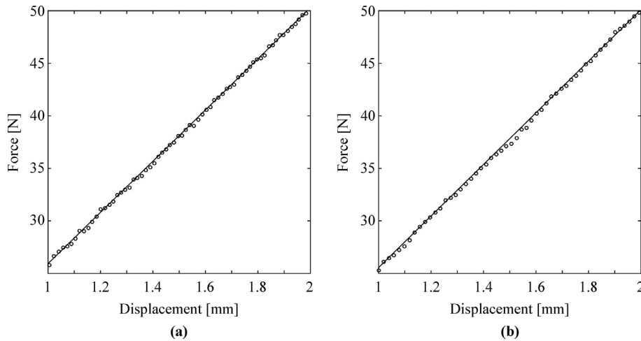
Fig. 7. Measured load-deflection characteristics of a linear helical spring. (a) Loading process data. (b) Unloading process data. Key: ○ representative measured data and — line of best fit.
