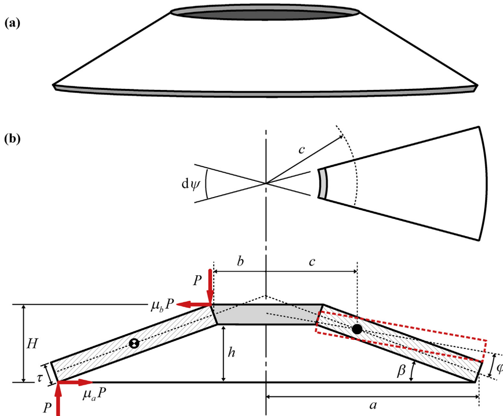
Fig. 1. Example case. (a) Coned disk spring with square edges; (b) top and cross section views of a coned disk spring with geometric parameters and loads: --- cross section deformed position, → edge contact force. Symbols are defined in the text and in Appendix A .
