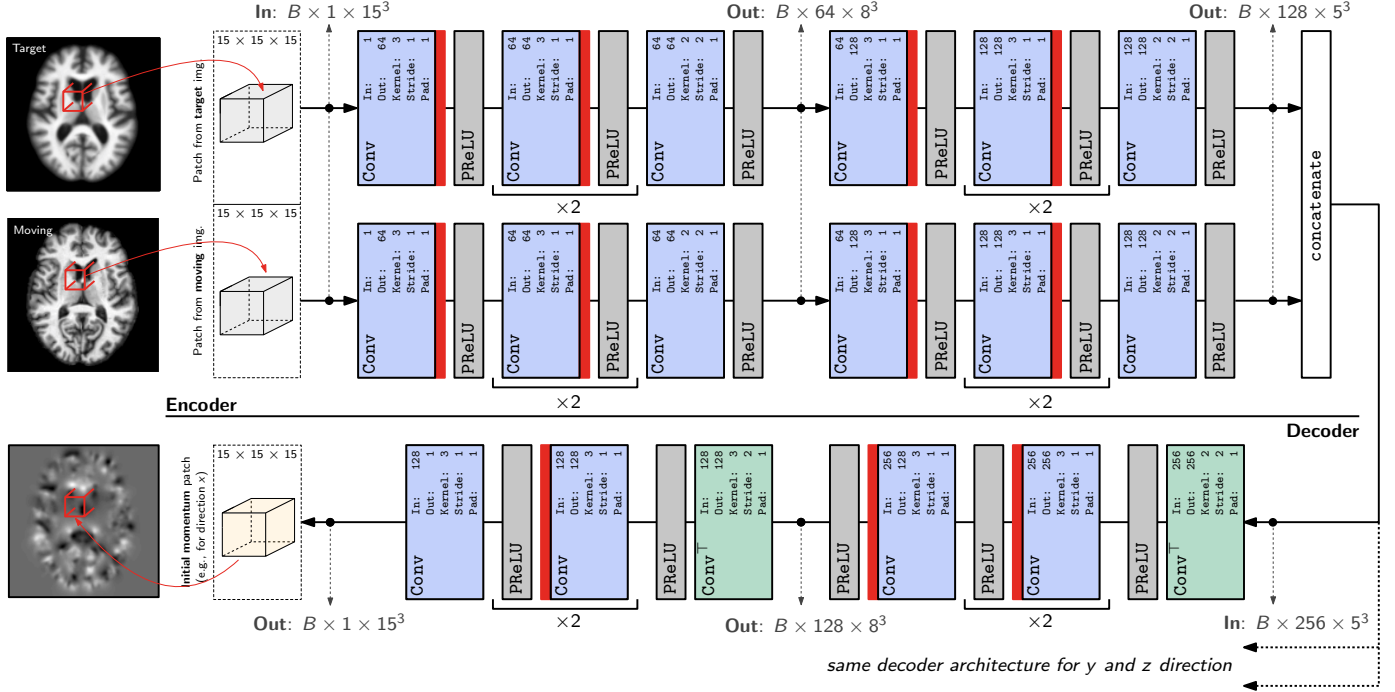
Figure 2: 3D (probabilistic) network architecture. The network takes two 3D patches from the moving and target image as the input, and outputs 3D initial momentum patches (one for each of the x, y and z dimensions respectively; for readability, only one decoder branch is shown in the figure). In case of the deterministic network, see Sec. 2.2.1, the dropout layers, illustrated by \blacksquare , are removed. Conv : 3D convolution layer. Conv T : 3D transposed convolution layer. Parameters for the Conv and Conv T layers: In : input channel. Out : output channel. Kernel : 3D filter kernel size in each dimension. Stride : stride for the 3D convolution. Pad : zero-padding added to the boundaries of the input patch. Note that in this illustration B denotes the batch size.
