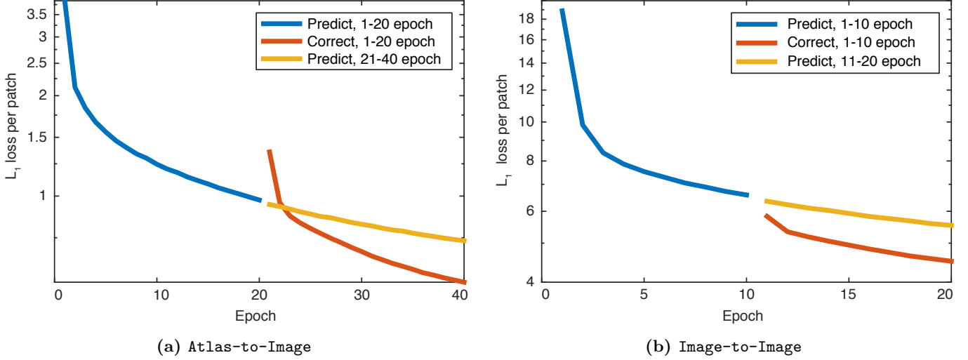
Figure 4: \log_{10} plot of l_1 training loss per patch. The loss is averaged across all iterations for every epoch for both the Atlas-to-Image case and the Image-to-Image case. The combined prediction + correction networks obtain a lower loss per patch than the loss obtained by simply training the prediction networks for more epochs.
