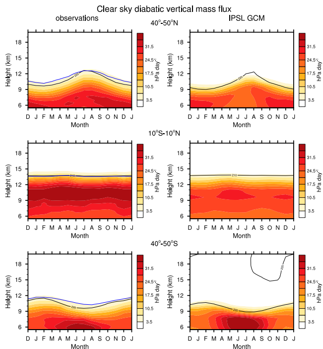
Fig. 2. Clear-sky diabatic vertical mass flux (shading) for indicated latitude bands as a function of calendar month and altitude. The black lines indicate the 220K isotherm ( Top and Bottom ) and 210K isotherm ( Middle ). The blue lines on all panels indicate the 20 ppmv water vapor isopleth. Results in the Left are derived from observations. Results in the Right are derived from the IPSL general circulation model (GCM).
