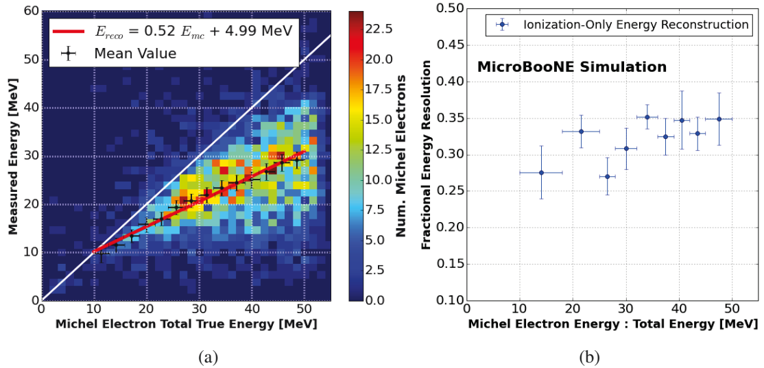
Figure 14. (a) reconstructed Michel electron ionization-only energy as a function of the true total Michel electron energy. (b) fractional energy resolution as a function of the true Michel electron energy. Error bars represent the uncertainty on the fit value.
