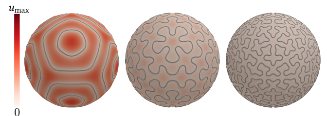
Fig. 3. Without penalizing length, a cut that seeks to minimize distortion will evolve into a curve reminiscent of space filling curves. Surface coloring indicates area distortion (here we explicitly enforce icosahedral symmetry).
