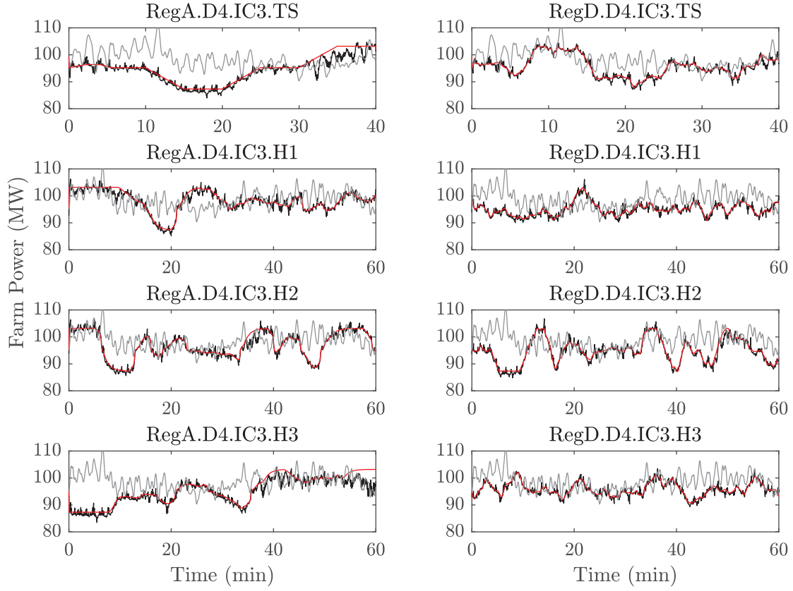
Figure 8. Power tracking performance of dynamic-model controlled wind farms comparing simulated farm power from a controlled LES wind farm model (—) an uncontrolled LES wind farm model (---), and power reference signals (—) for 4% derates and initial condition 3.
