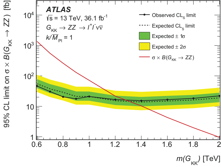
Figure 10: The upper limits at 95% CL on cross section times branching ratio \sigma \times B(G_{KK} \rightarrow ZZ) for a KK graviton produced with k/\bar{M}_{Pl} = 1 . The green and yellow bands give the \pm 1\sigma and \pm 2\sigma uncertainties in the expected limits. The predicted production cross section times branching ratio as a function of the G_{KK} mass m(G_{KK}) is shown by the red solid line.
