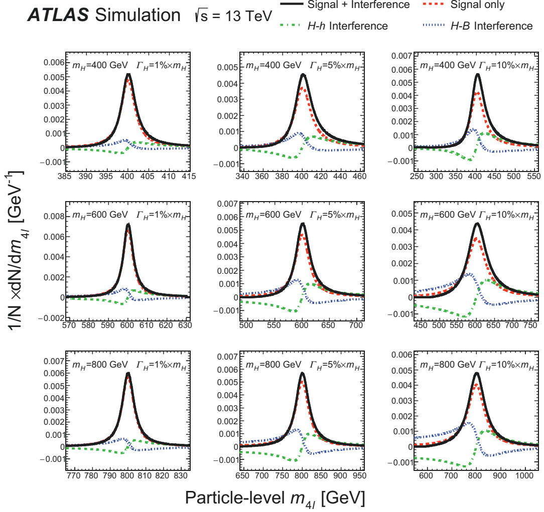
Figure 2: Particle-level four-lepton mass m_{4\ell} model for signal only (red), H - h interference (green), H - B interference (blue) and the sum of the three processes (black). Three values of the resonance mass m_H (400, 600, 800 GeV) are chosen, as well as three values of the resonance width \Gamma_H (1%, 5%, 10% of m_H ). The signal cross section, which determines the relative contribution of the signal and interference, is taken to be the cross section of the expected limit for each combination of m_H and \Gamma_H . The full model (black) is finally normalised to unity and the other contributions are scaled accordingly.
