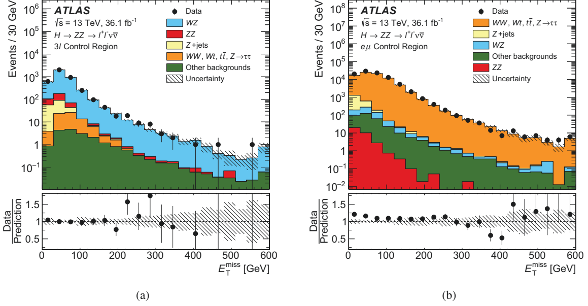
Figure 3: Missing transverse momentum E_T^{\text{miss}} distribution (a) for events in the 3\ell control region as defined in the text and (b) for e^\pm\mu^\pm lepton pairs after applying the dilepton invariant mass requirement, before applying the rest of the control region selection. The backgrounds are determined following the description in Section 6.2 and the last bin includes the overflow. The small excess below 120 GeV in (b) arises from Z + \text{jets} background which is here taken from simulation, and lies outside the control region. The error bars on the data points indicate the statistical uncertainty, while the systematic uncertainty in the prediction is shown by the hatched band. The lower panels show the ratio of data to prediction.
