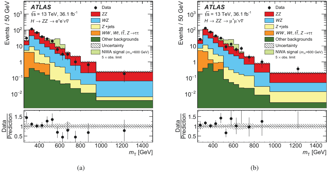
Figure 5: Transverse mass m_T distribution in the \ell^+\ell^-\nu\bar{\nu} search for (a) the electron channel and (b) the muon channel, including events from both the ggF-enriched and the VBF-enriched categories. The backgrounds are determined following the description in Section 6.2 and the last bin includes the overflow. The simulated m_H = 600 GeV signal is normalized to a cross section corresponding to five times the observed limit given in Section 8.3.1. The error bars on the data points indicate the statistical uncertainty and markers are drawn at the bin centre. The systematic uncertainty in the prediction is shown by the hatched band. The lower panels show the ratio of data to prediction.
