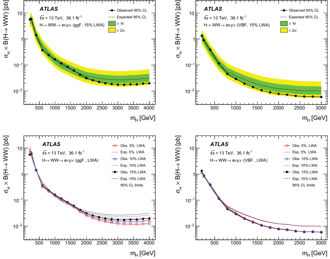
Figure 9: Upper limits at 95% CL on the Higgs boson production cross section times branching fraction \sigma_H \times B(H \rightarrow WW) in the \nu_e \nu_\mu channel, for a signal with a width of 15% of the mass (top) and the comparison of three different widths (bottom) for the ggF (left) and VBF (right) production. The inner and outer bands show the \pm 1\sigma and \pm 2\sigma ranges around the expected limit.
