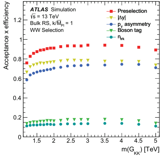
(c) Bulk RS model, k/\overline{M}_{Pl} = 1
