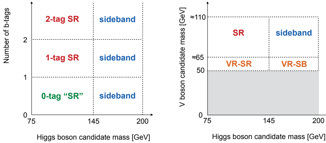
Figure 1: Illustration of the sideband and validation regions, showing orthogonal slices through the space defined by the masses of the two boson candidates and the number of b -tags.
