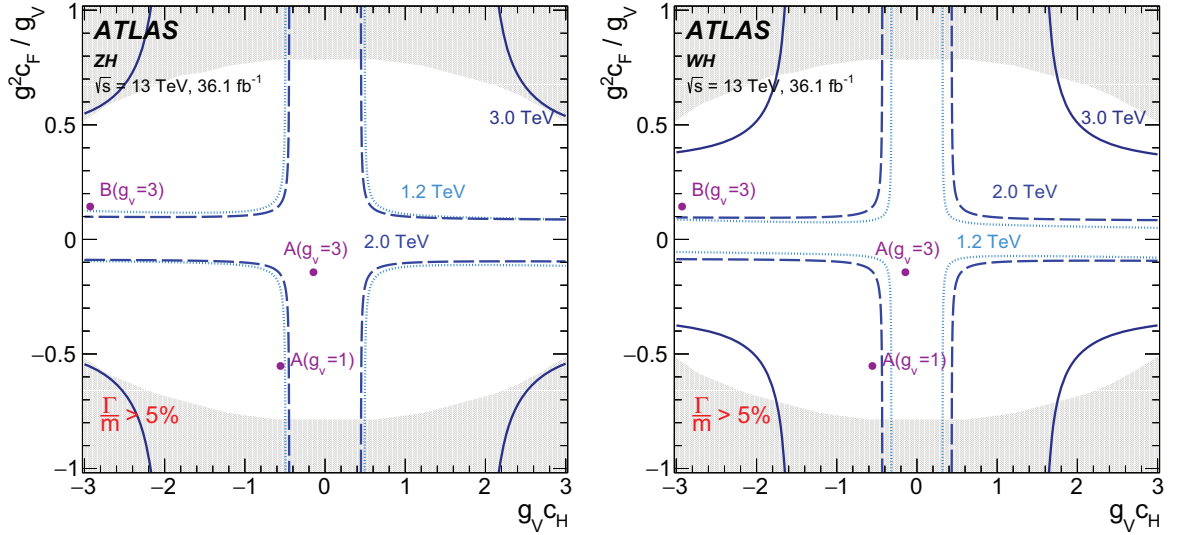
Figure 5: Limits in the g^2 c_F / g_V vs. g_V c_H plane for several resonance masses for the (left) ZH and (right) WH channels. Areas outside the curves are excluded. The benchmark model points are also shown. Coupling values for which the resonance width \Gamma/m > 5\% are shown in grey, as these regions may not be well described by the narrow width approximation.
