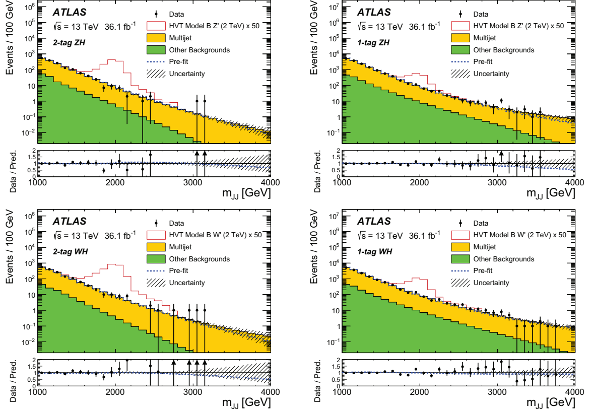
Figure 3: The m_{JJ} distributions in the VH signal regions for data (points) and background estimate (histograms) after the likelihood fit for events in the (left) 2-tag and (right) 1-tag categories. The pre-fit background expectation is given by the blue dashed line. The expected signal distributions (multiplied by 50) for a HVT benchmark Model B V' boson with 2 TeV mass are also shown. In the data/prediction ratio plots, arrows indicate off-scale points.
