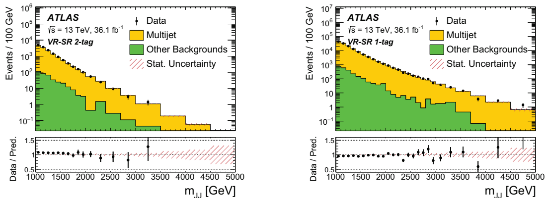
Figure 2: The m_{JJ} distribution in the signal-region-like validation region in the (left) 2-tag (right) 1-tag samples, compared to the predicted background. The uncertainty band corresponds to the statistical uncertainty on the multijet model.
