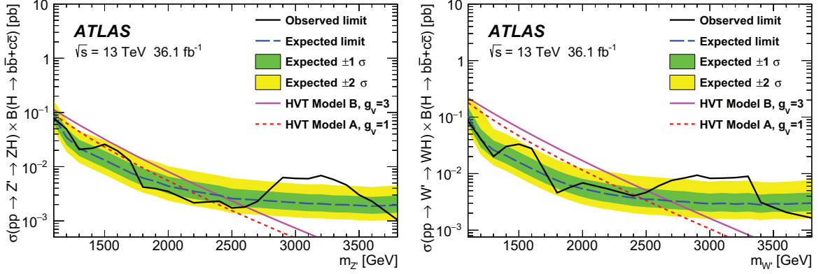
Figure 4: The observed and expected cross-section upper limits at the 95% confidence level for \sigma(pp \rightarrow V' \rightarrow VH) \times B(H \rightarrow (b\bar{b} + c\bar{c})) , assuming SM branching ratios, in Model A and Model B in the (left) ZH and (right) WH signal regions. The red and magenta curves show the predicted cross-sections as a function of resonance mass for the models considered.
