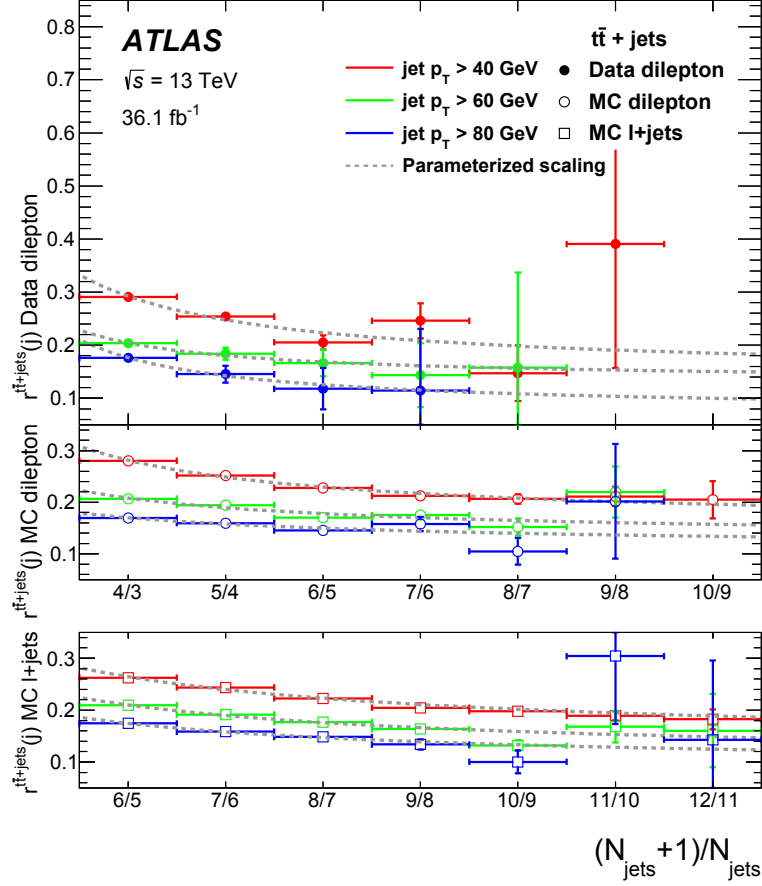
Figure 5: The ratio of the number of events with (j+1) jets to the number with j jets in dileptonic and semileptonic t\bar{t} + \text{jets} events, used to validate the jet-scaling parameterization. Each panel shows the ratio for data or MC simulation with the fitted parameterization overlaid as a line. In the case of pure “staircase scaling”, the shown ratio would be a constant. The uncertainties shown are statistical.
