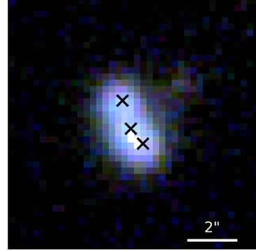
Figure 1. PS J0630–1201 as a g, r, i PS colour composite. The single band stacked images were obtained from the PS cutout server ( http://pslimages.stsci.edu/cgi-bin/pslcutouts ). The black crosses mark the positions of overlapping objects from the Gaia catalogue. North is up and East is to the left.
