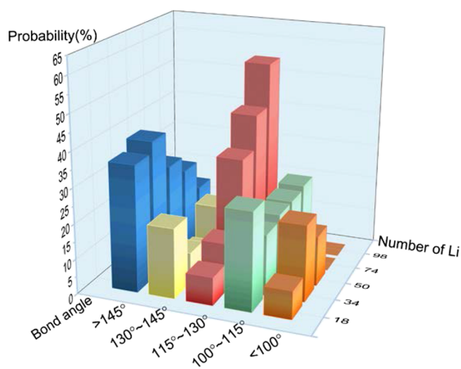
Figure 5. Bond angle distribution of C–C–C, Si–C–C, and Si–C–Si clusters in five representative \text{Li}_x\text{SiOC} compositions. The salient features are that the probability of bond angles larger than 145^\circ steadily decreases, whereas the distribution of bond angles between 115^\circ and 130^\circ increases significantly upon lithiation. This demonstrates the geometry optimization of C atoms toward the \text{sp}^2 type coordinated by Li insertion.
