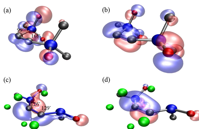
Figure 6. Evolution of two MOs contributed by two centered C atoms in a Si–C–C–Si cluster. (a) Before lithiation, the p_y orbitals of the two C atoms overlap to form one \pi_y -type MO. (b) Similarly, two p_z atomic orbitals overlap to form the \pi_z orbital. (c) After lithiation, the original \pi_y orbital is perturbed by the virtual orbital of the nearby Li atoms (not shown in the diagram) and is split into two atomic orbitals in different orientations, which promotes the formation of the hybrid \text{sp}^2 orbital. (d) In comparison, there is no obvious difference in \pi_z which remains perpendicular to the \text{sp}^2 hybrid planar orbital before and after lithiation.
