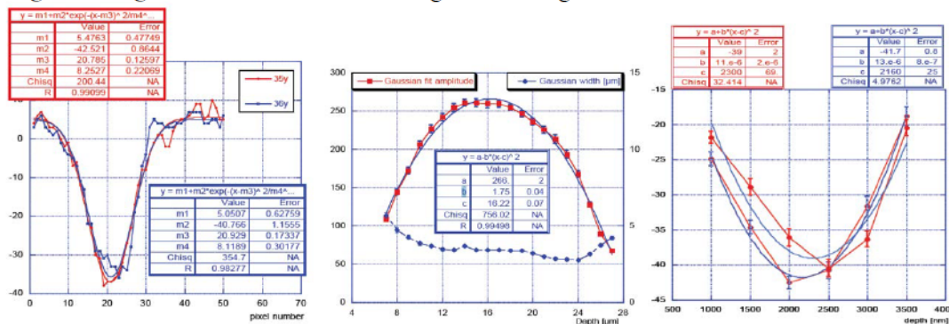
Figure 4: Left: Gaussian fit to two dark field Airy function slices, whose amplitude (m1) is used to find the scatterer depth. Center: amplitude vs. depth fitting with dark field (20x magnification) used to determine the depth (C). Right: Two bright field (50x magnification) amplitude vs. depth fittings, a slightly better depth resolution is achieved.
