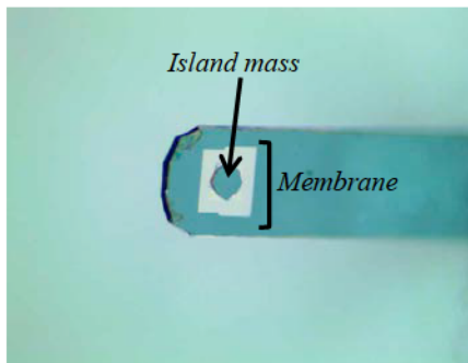
Figure 5: Pictured is an actual sample in our possession that was manufactured by Chao Shiuh's group at National Tsing Hua University. The membrane and island mass are at the end of a long stem to prevent damage during shipping. The island mass has a diameter ~380 microns. The exposed membrane area is ~890 microns, with a thickness of ~100nm. We will glue the entire stem to our fused silica stage using the UV activated epoxy, with minimal losses.
