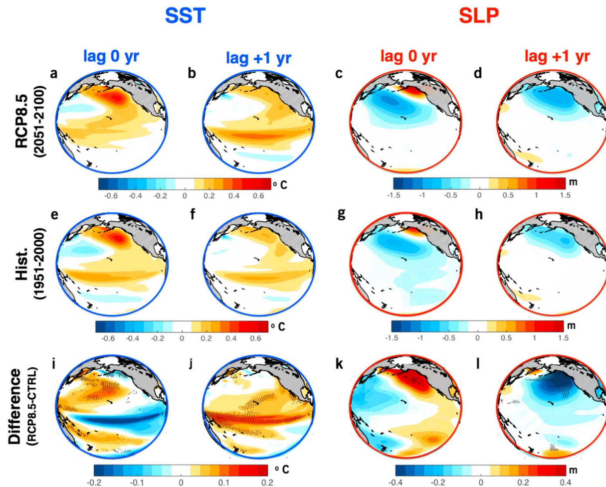
Figure 4. Evolution of the NEP warm events and related atmospheric forcing of the CESM-LENS ensemble mean. Regression maps of OEI (of 1^{\circ}\text{C} ) to SSTa and SLPa with 0 and +1 year lag for the 50 years of (a–d) RCP8.5 and (e–h) historical scenario. Difference maps between the (i–l) RCP8.5 and historical scenario (RCP8.5 minus historical). Stippling indicates regions where the difference of two regression coefficients is statistically significant above the 90% confidence level as determined by a two-tailed Student's t test.
