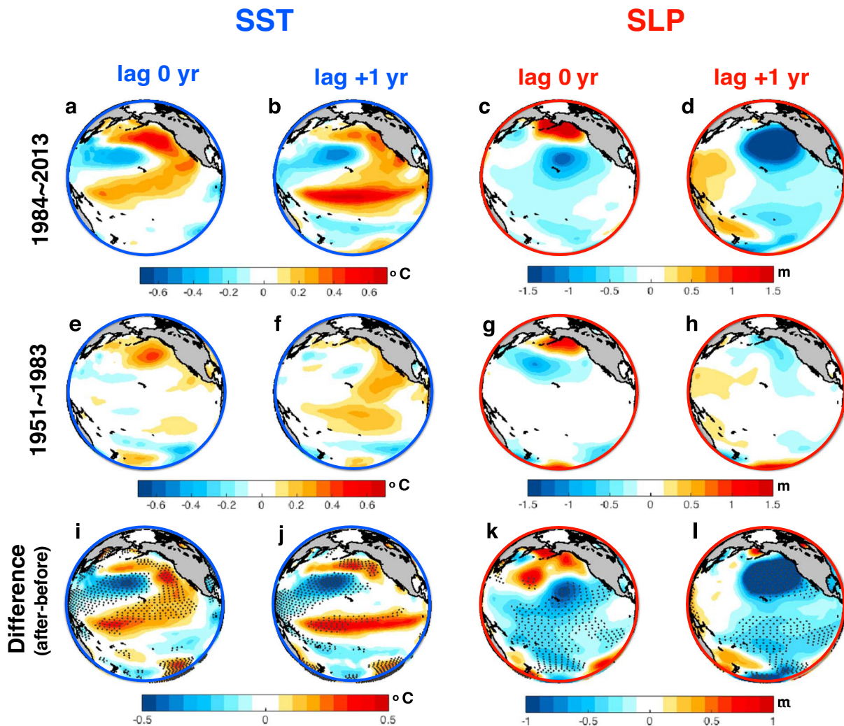
Figure 2. Evolution of observed NEP warm temperature events and related atmospheric forcing. Regression maps of OEI (of 1^{\circ}\text{C} to SSTa and SLPa with 0 and +1 year lag during the period of (a–d) 1984–2013, (e–h) 1951–1983. Difference maps between the (i–l) two periods (recent minus previous). Stippling indicates regions where the difference of two regression coefficients is statistically significant above the 90% confidence level as determined by a two-tailed Student's t test.
