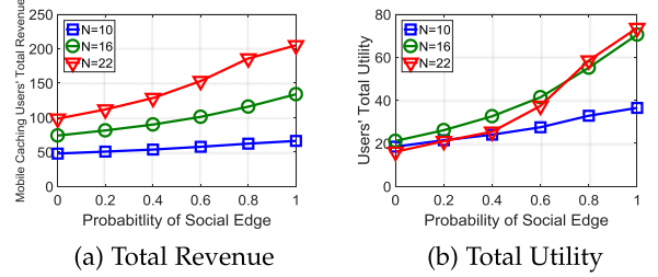
Fig. 8. Effect from RUs.
