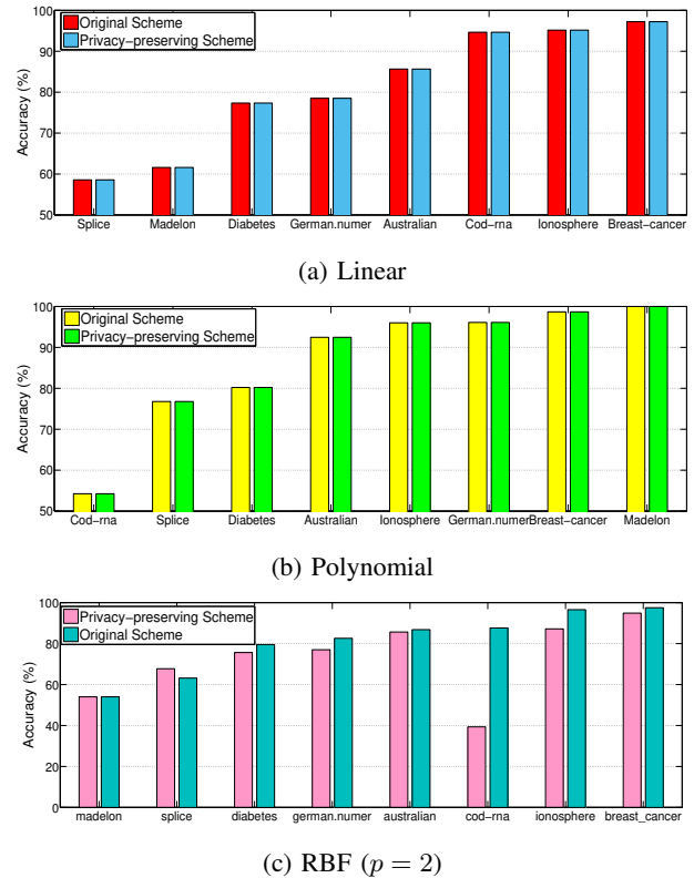
Fig. 8: Classification Accuracy
