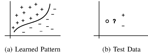
Fig. 4: Data Classification
