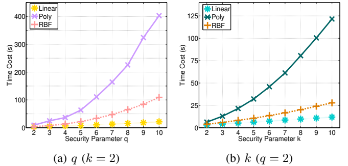
Fig. 10: Computational Cost with Different Security Parameter
