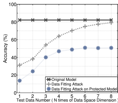
Fig. 12: Attack & Protection with Different Test Data
